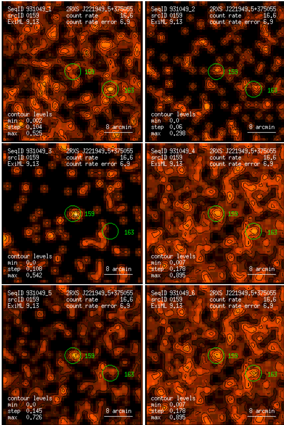
Figure 159: RASS 931049: detection 0159: band rate images, Gaussian filter: (1) PSPC channels 11 – 41, (2) 52 – 90, (3) 91 – 201, (4) 11 – 235, (5) 52 – 201, (6) 11 – 201. Broad band rates in counts/ks. Band rate contour levels in counts/ks/arcmin 2 .
