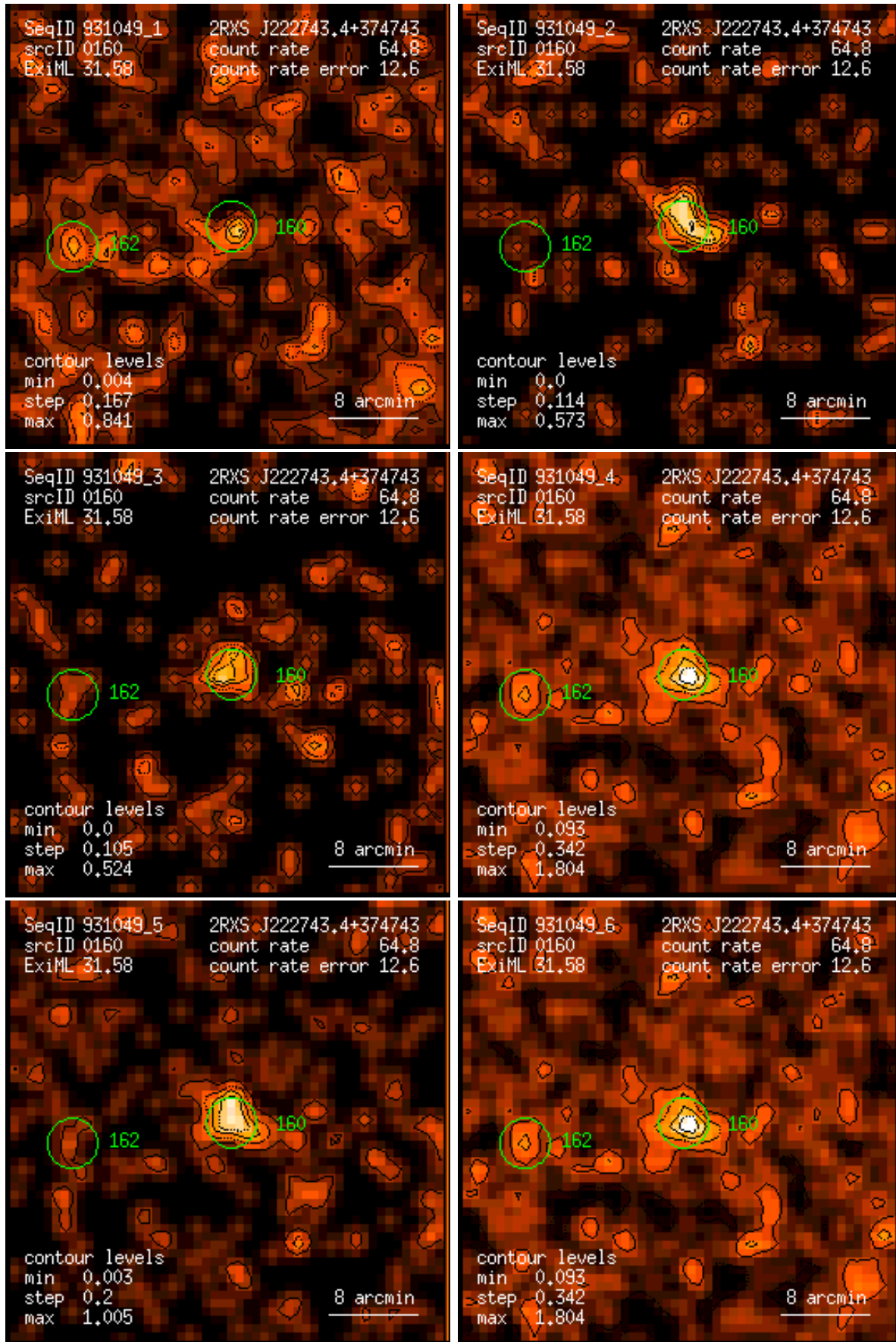
Figure 160: RASS 931049: detection 0160: band rate images, Gaussian filter: (1) PSPC channels 11 – 41, (2) 52 – 90, (3) 91 – 201, (4) 11 – 235, (5) 52 – 201, (6) 11 – 201. Broad band rates in counts/ks. Band rate contour levels in counts/ks/arcmin 2 .
