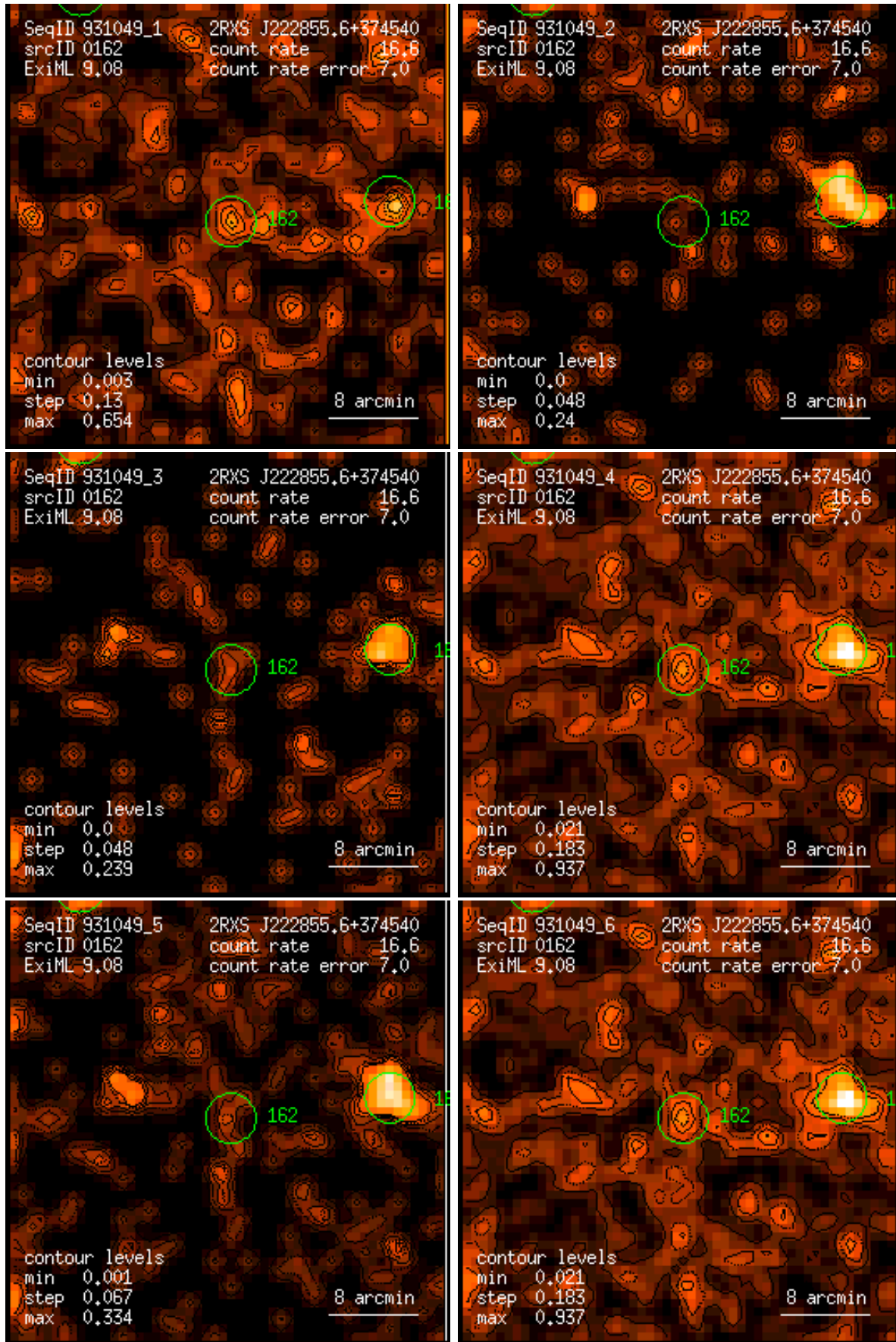
Figure 162: RASS 931049: detection 0162: band rate images, Gaussian filter: (1) PSPC channels 11 – 41, (2) 52 – 90, (3) 91 – 201, (4) 11 – 235, (5) 52 – 201, (6) 11 – 201. Broad band rates in counts/ks. Band rate contour levels in counts/ks/arcmin 2 .
