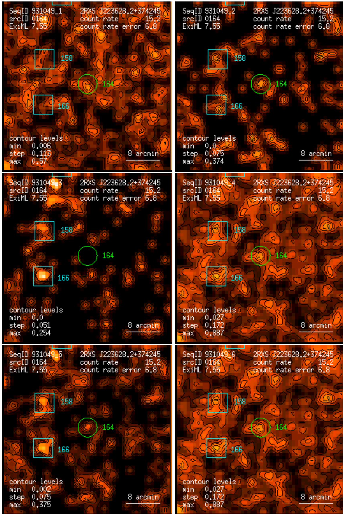
Figure 164: RASS 931049: detection 0164: band rate images, Gaussian filter: (1) PSPC channels 11 – 41, (2) 52 – 90, (3) 91 – 201, (4) 11 – 235, (5) 52 – 201, (6) 11 – 201. Broad band rates in counts/ks. Band rate contour levels in counts/ks/arcmin 2 .
