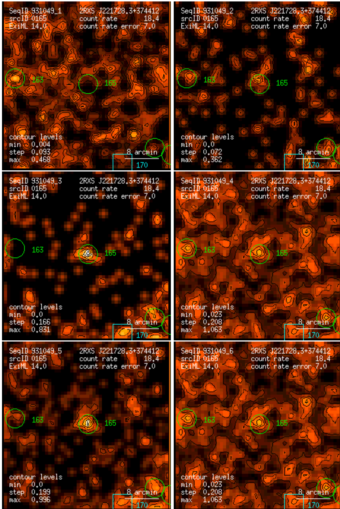
Figure 165: RASS 931049: detection 0165: band rate images, Gaussian filter: (1) PSPC channels 11 – 41, (2) 52 – 90, (3) 91 – 201, (4) 11 – 235, (5) 52 – 201, (6) 11 – 201. Broad band rates in counts/ks. Band rate contour levels in counts/ks/arcmin 2 .
