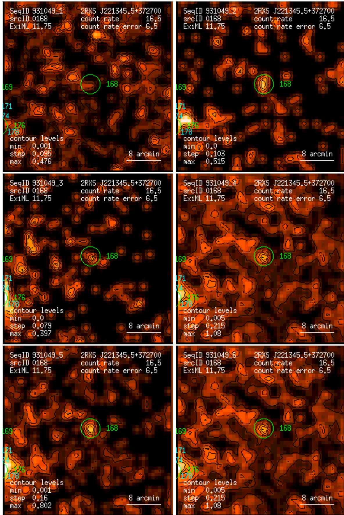
Figure 168: RASS 931049: detection 0168: band rate images, Gaussian filter: (1) PSPC channels 11 – 41, (2) 52 – 90, (3) 91 – 201, (4) 11 – 235, (5) 52 – 201, (6) 11 – 201. Broad band rates in counts/ks. Band rate contour levels in counts/ks/arcmin 2 .
