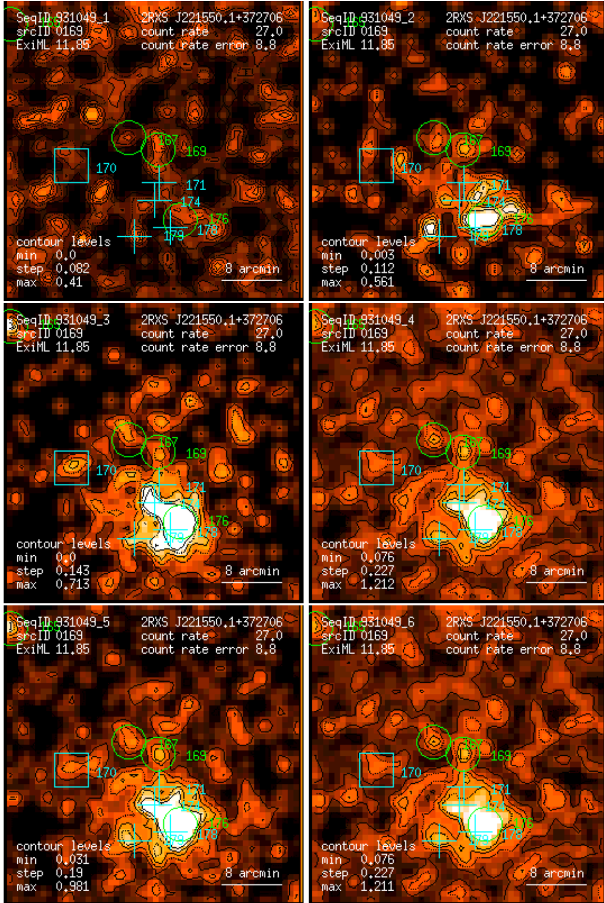
Figure 169: RASS 931049: detection 0169: band rate images, Gaussian filter: (1) PSPC channels 11 – 41, (2) 52 – 90, (3) 91 – 201, (4) 11 – 235, (5) 52 – 201, (6) 11 – 201. Broad band rates in counts/ks. Band rate contour levels in counts/ks/arcmin 2 .
