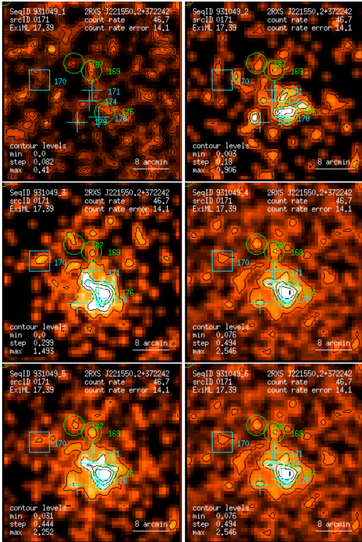
Figure 171: RASS 931049: detection 0171: band rate images, Gaussian filter: (1) PSPC channels 11 – 41, (2) 52 – 90, (3) 91 – 201, (4) 11 – 235, (5) 52 – 201, (6) 11 – 201. Broad band rates in counts/ks. Band rate contour levels in counts/ks/arcmin 2 .
