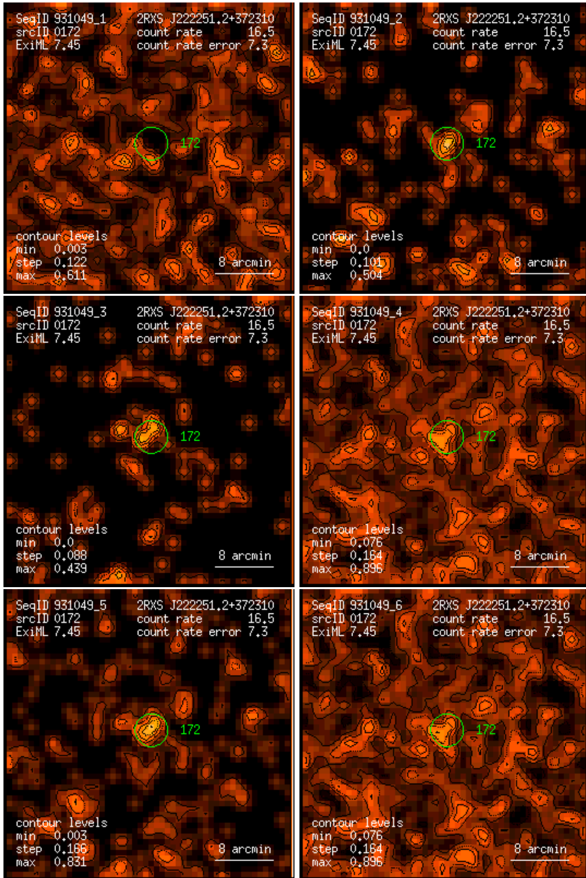
Figure 172: RASS 931049: detection 0172: band rate images, Gaussian filter: (1) PSPC channels 11 – 41, (2) 52 – 90, (3) 91 – 201, (4) 11 – 235, (5) 52 – 201, (6) 11 – 201. Broad band rates in counts/ks. Band rate contour levels in counts/ks/arcmin 2 .
