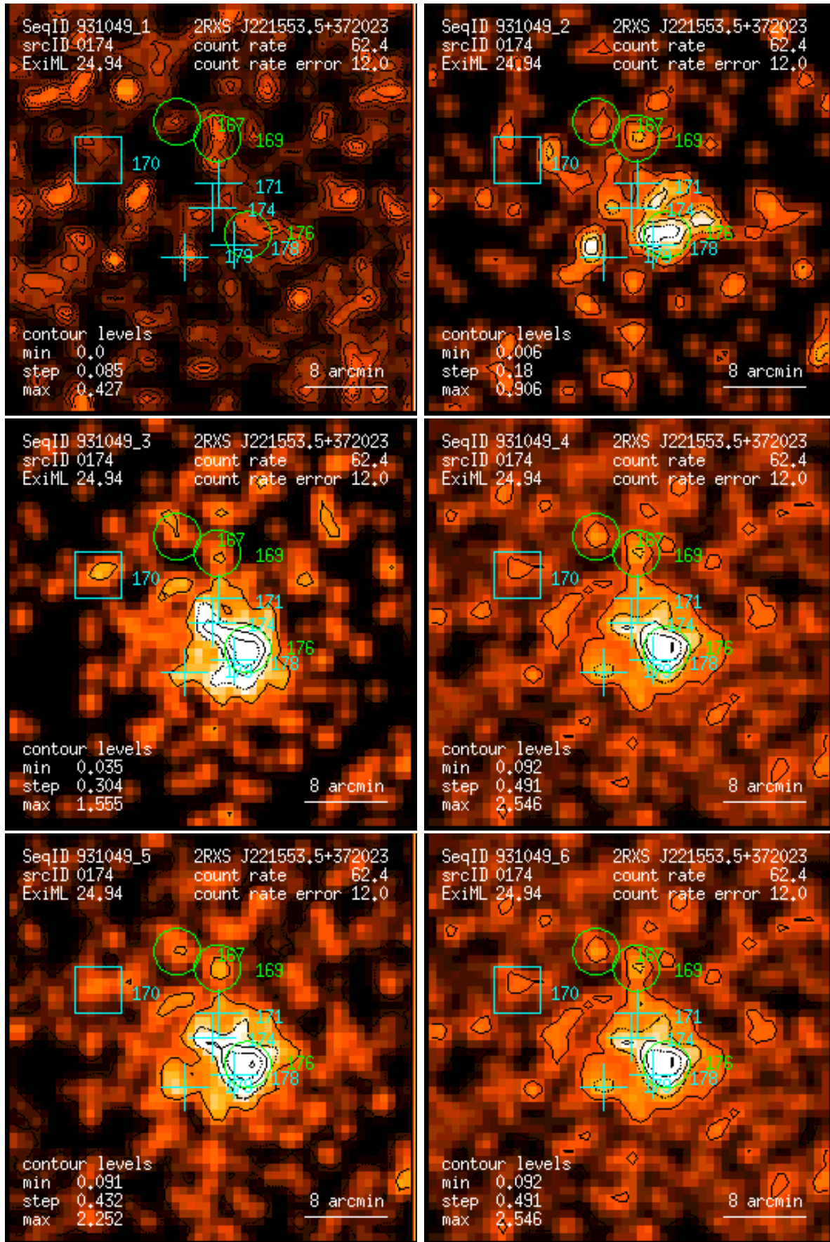
Figure 174: RASS 931049: detection 0174: band rate images, Gaussian filter: (1) PSPC channels 11 – 41, (2) 52 – 90, (3) 91 – 201, (4) 11 – 235, (5) 52 – 201, (6) 11 – 201. Broad band rates in counts/ks. Band rate contour levels in counts/ks/arcmin 2 .
