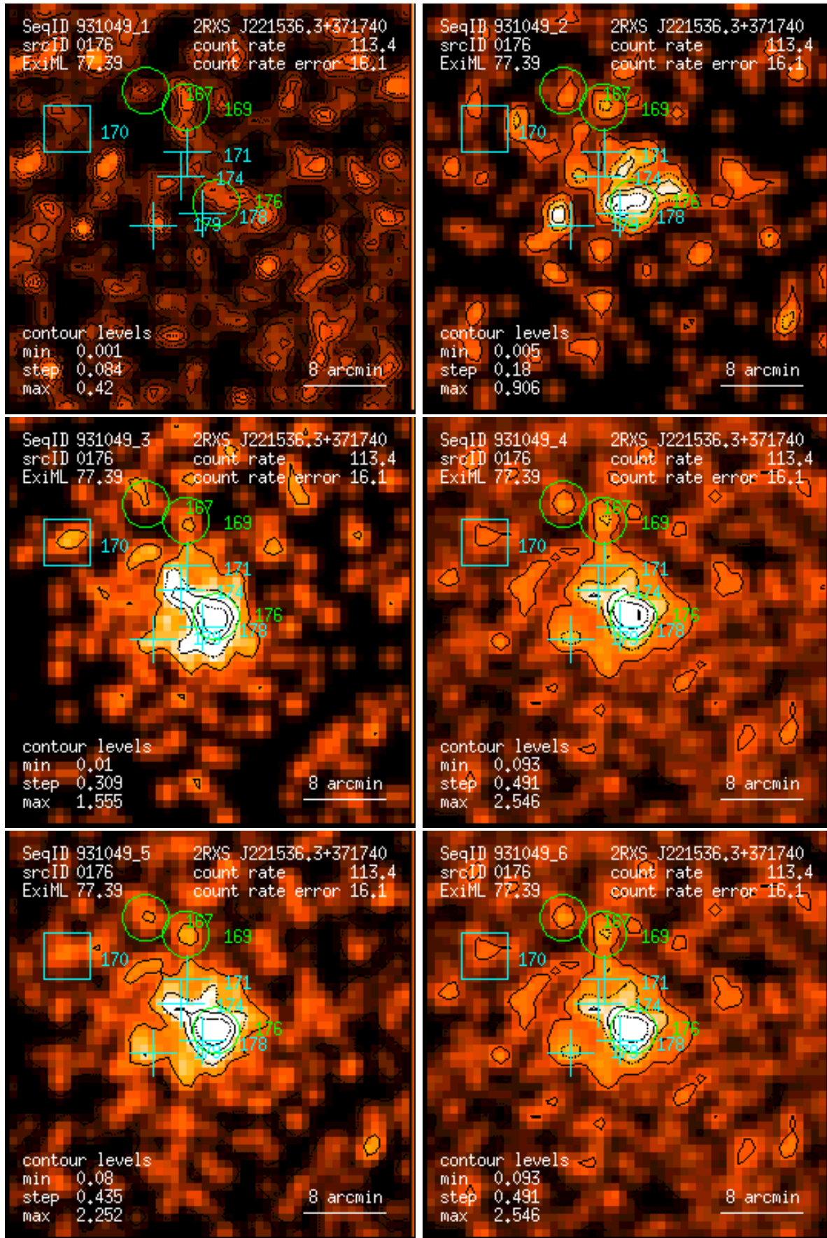
Figure 176: RASS 931049: detection 0176: band rate images, Gaussian filter: (1) PSPC channels 11 – 41, (2) 52 – 90, (3) 91 – 201, (4) 11 – 235, (5) 52 – 201, (6) 11 – 201. Broad band rates in counts/ks. Band rate contour levels in counts/ks/arcmin 2 .
