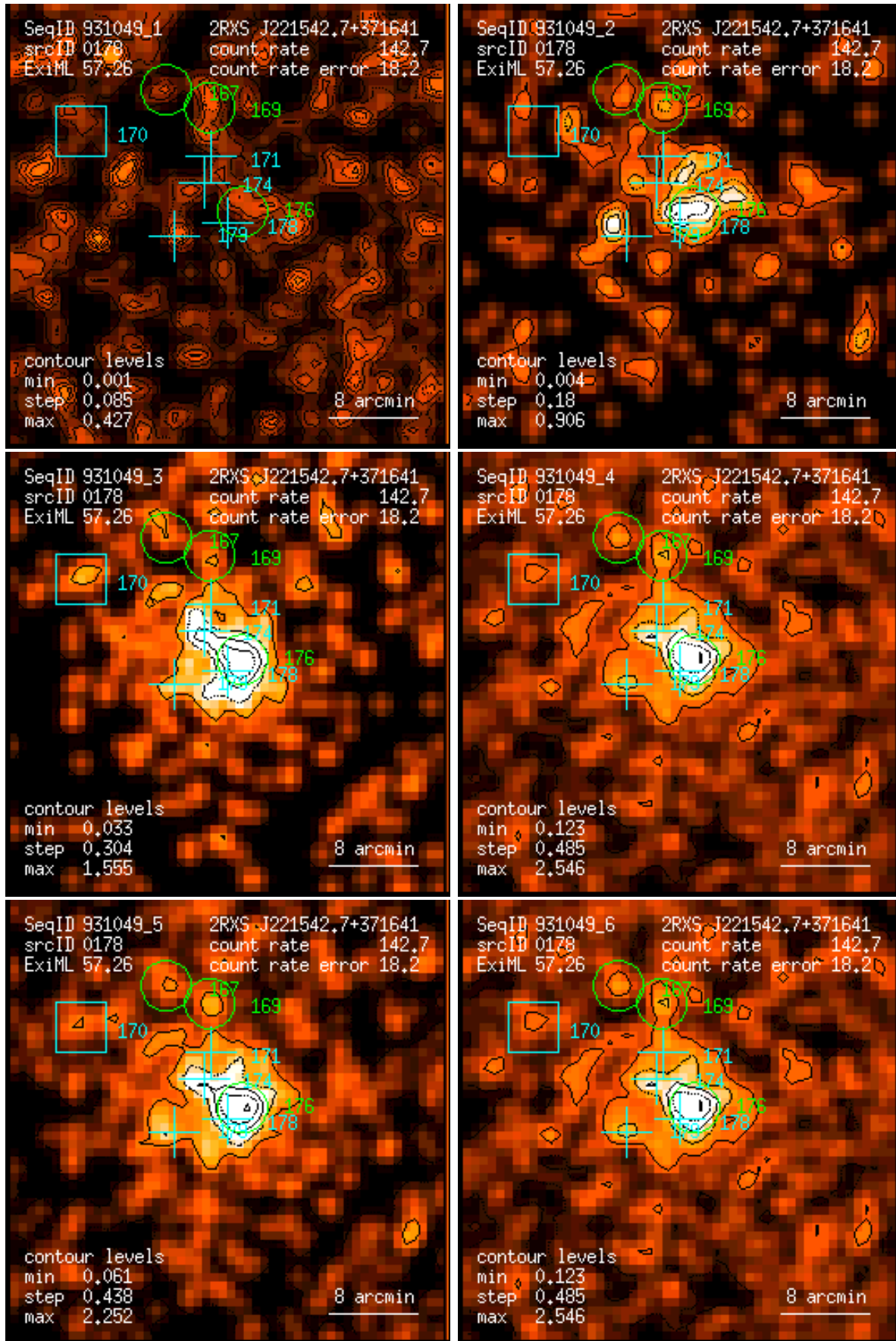
Figure 178: RASS 931049: detection 0178: band rate images, Gaussian filter: (1) PSPC channels 11 – 41, (2) 52 – 90, (3) 91 – 201, (4) 11 – 235, (5) 52 – 201, (6) 11 – 201. Broad band rates in counts/ks. Band rate contour levels in counts/ks/arcmin 2 .
