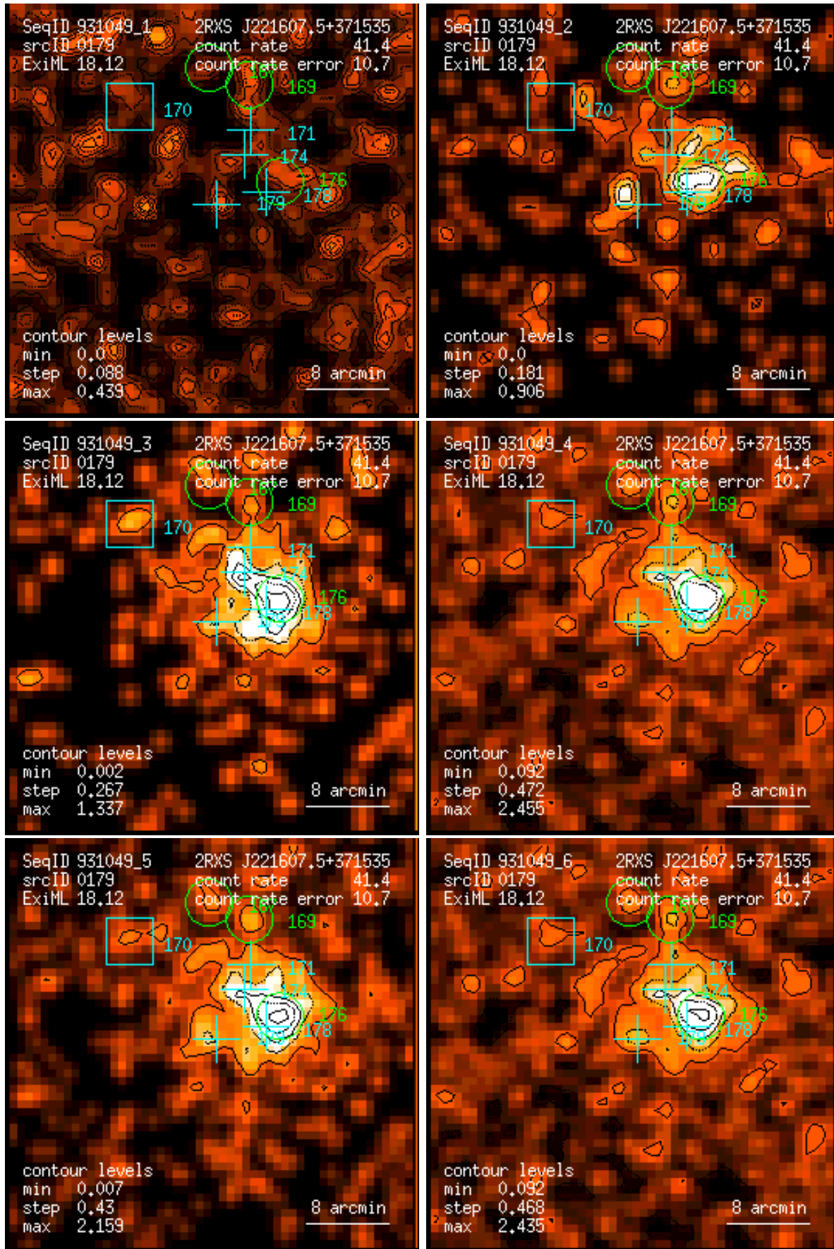
Figure 179: RASS 931049: detection 0179: band rate images, Gaussian filter: (1) PSPC channels 11 – 41, (2) 52 – 90, (3) 91 – 201, (4) 11 – 235, (5) 52 – 201, (6) 11 – 201. Broad band rates in counts/ks. Band rate contour levels in counts/ks/arcmin 2 .
