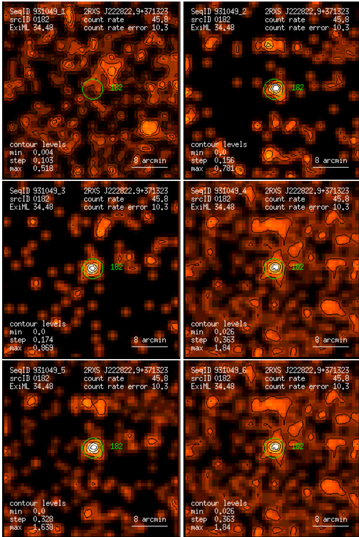
Figure 182: RASS 931049: detection 0182: band rate images, Gaussian filter: (1) PSPC channels 11 – 41, (2) 52 – 90, (3) 91 – 201, (4) 11 – 235, (5) 52 – 201, (6) 11 – 201. Broad band rates in counts/ks. Band rate contour levels in counts/ks/arcmin 2 .
