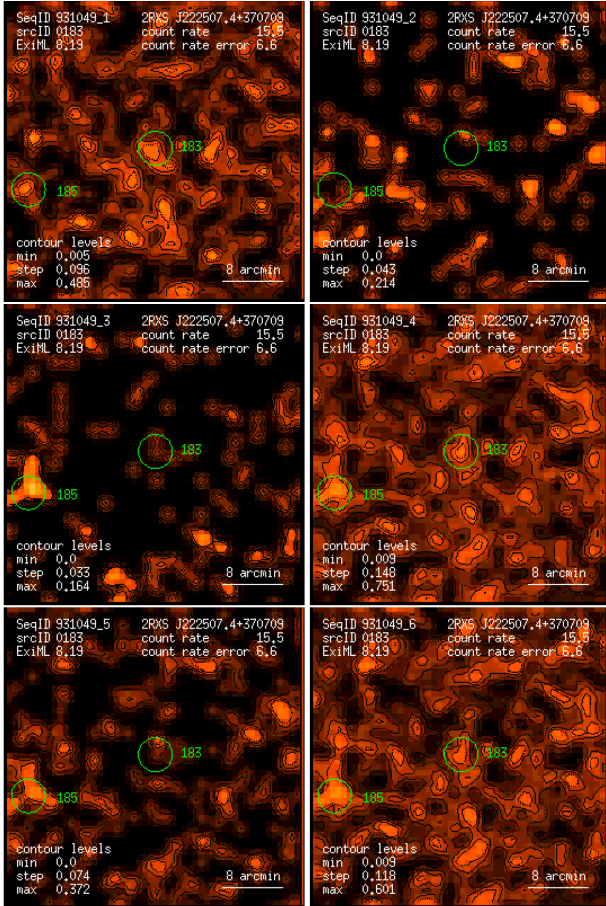
Figure 183: RASS 931049: detection 0183: band rate images, Gaussian filter: (1) PSPC channels 11 – 41, (2) 52 – 90, (3) 91 – 201, (4) 11 – 235, (5) 52 – 201, (6) 11 – 201. Broad band rates in counts/ks. Band rate contour levels in counts/ks/arcmin 2 .
