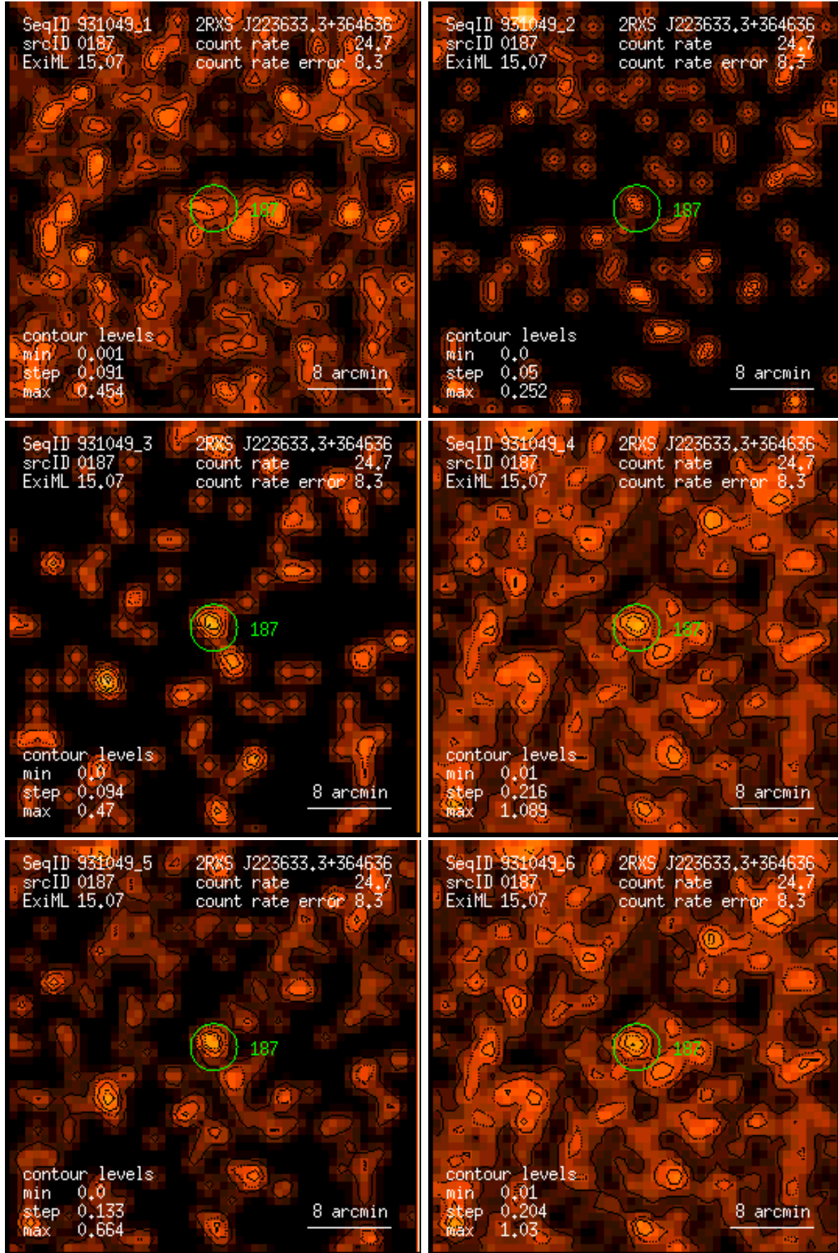
Figure 187: RASS 931049: detection 0187: band rate images, Gaussian filter: (1) PSPC channels 11 – 41, (2) 52 – 90, (3) 91 – 201, (4) 11 – 235, (5) 52 – 201, (6) 11 – 201. Broad band rates in counts/ks. Band rate contour levels in counts/ks/arcmin 2 .
