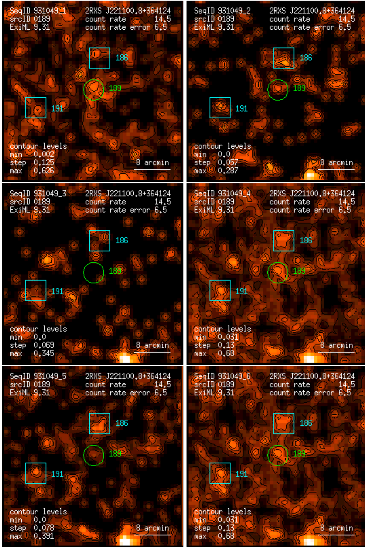
Figure 189: RASS 931049: detection 0189: band rate images, Gaussian filter: (1) PSPC channels 11 – 41, (2) 52 – 90, (3) 91 – 201, (4) 11 – 235, (5) 52 – 201, (6) 11 – 201. Broad band rates in counts/ks. Band rate contour levels in counts/ks/arcmin 2 .
