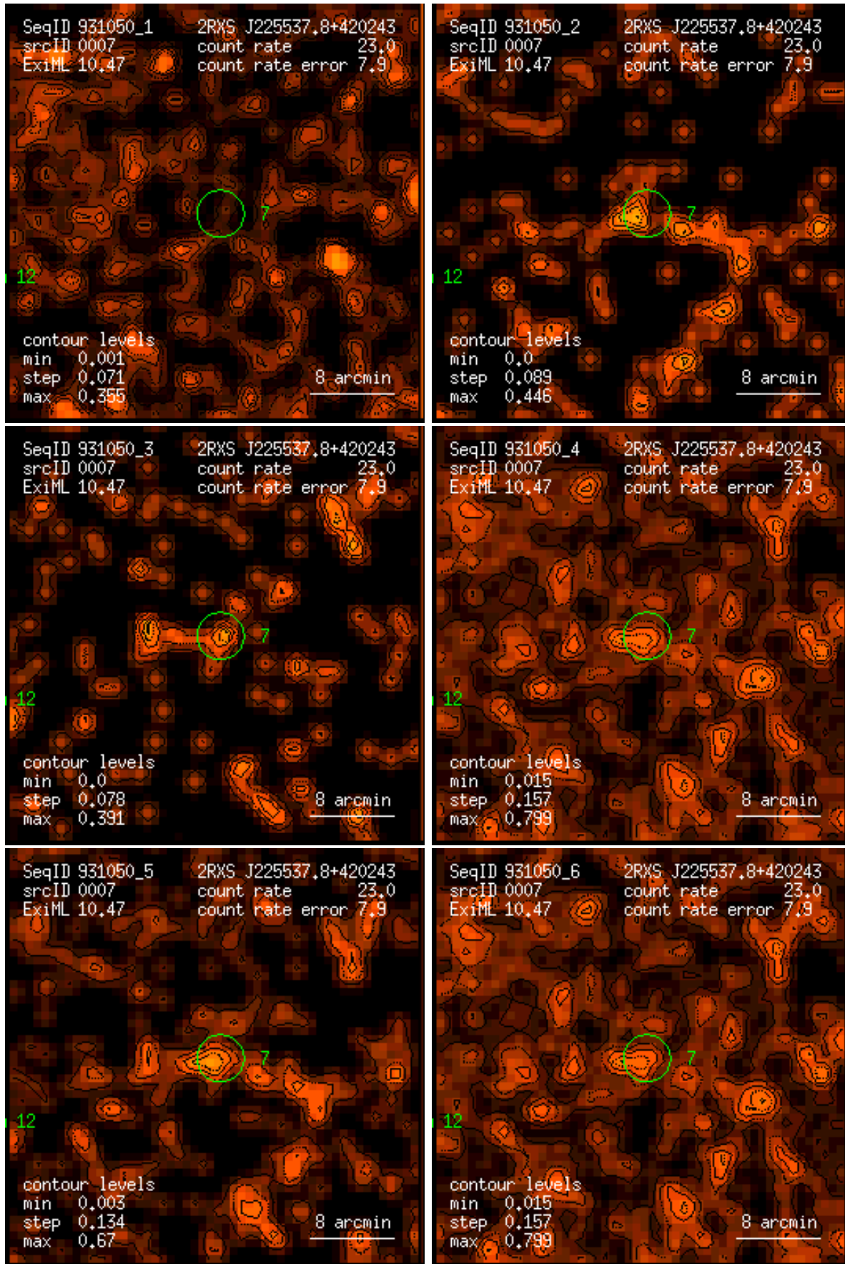
Figure 7: RASS 931050: detection 0007: band rate images, Gaussian filter: (1) PSPC channels 11 – 41, (2) 52 – 90, (3) 91 – 201, (4) 11 – 235, (5) 52 – 201, (6) 11 – 201. Broad band rates in counts/ks. Band rate contour levels in counts/ks/arcmin 2 .
