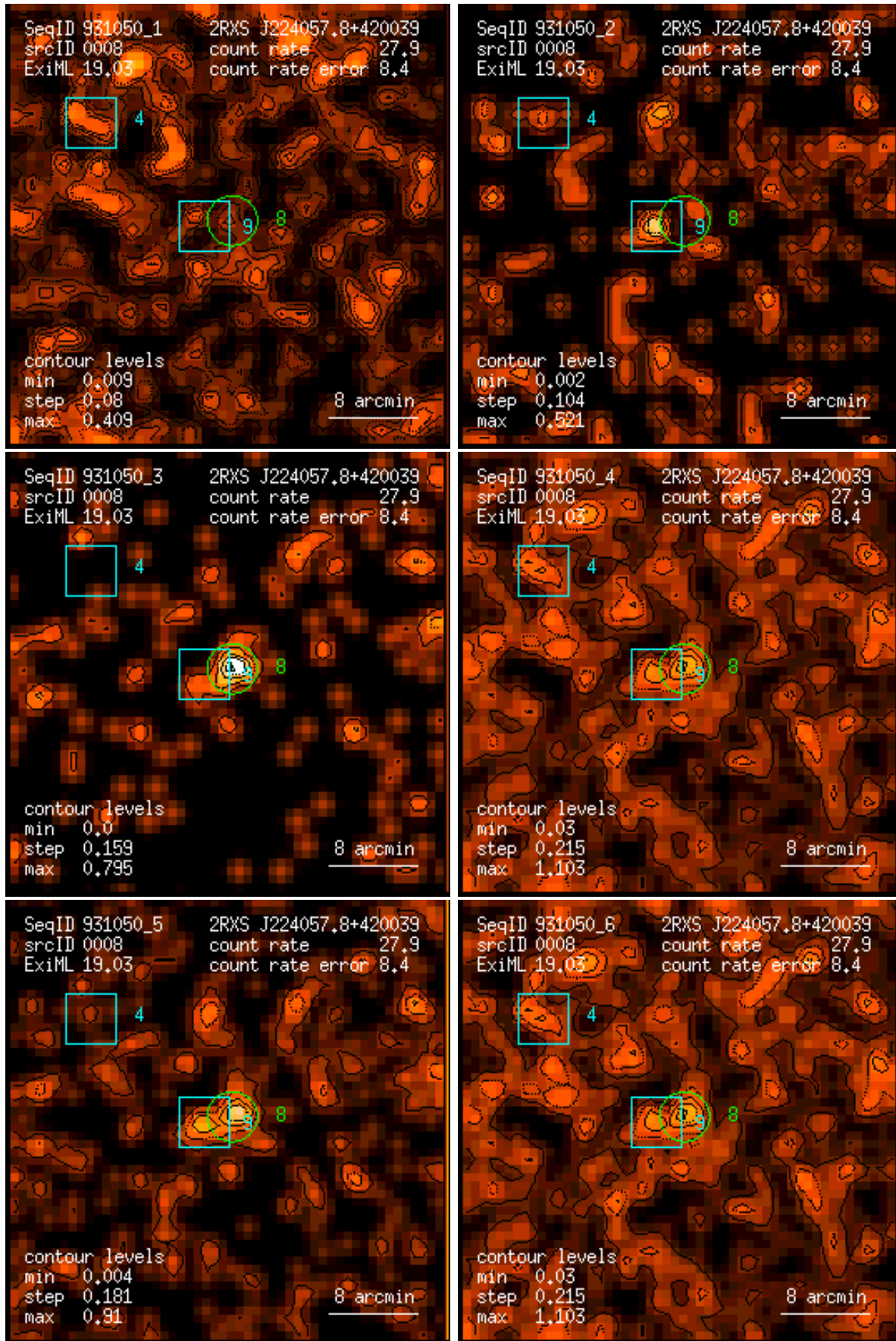
Figure 8: RASS 931050: detection 0008: band rate images, Gaussian filter: (1) PSPC channels 11 – 41, (2) 52 – 90, (3) 91 – 201, (4) 11 – 235, (5) 52 – 201, (6) 11 – 201. Broad band rates in counts/ks. Band rate contour levels in counts/ks/arcmin 2 .
