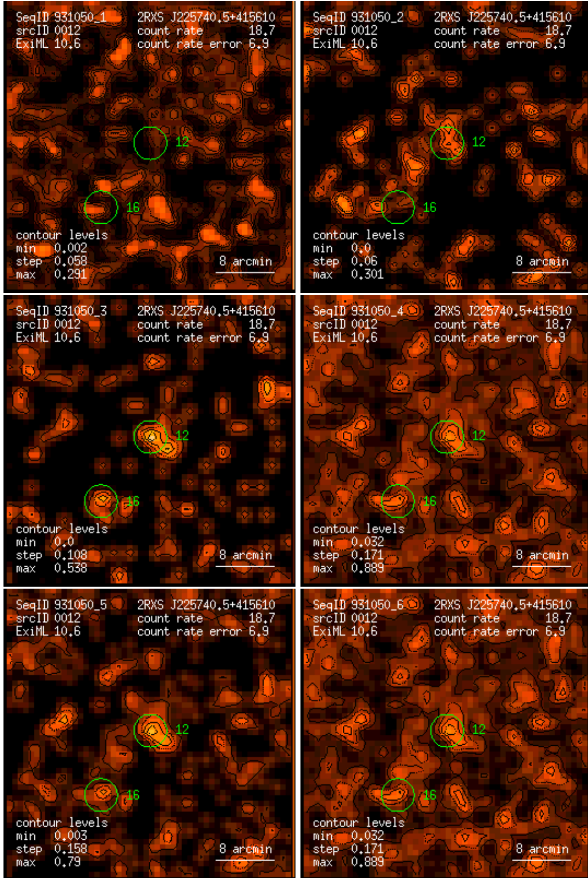
Figure 12: RASS 931050: detection 0012: band rate images, Gaussian filter: (1) PSPC channels 11 – 41, (2) 52 – 90, (3) 91 – 201, (4) 11 – 235, (5) 52 – 201, (6) 11 – 201. Broad band rates in counts/ks. Band rate contour levels in counts/ks/arcmin 2 .
