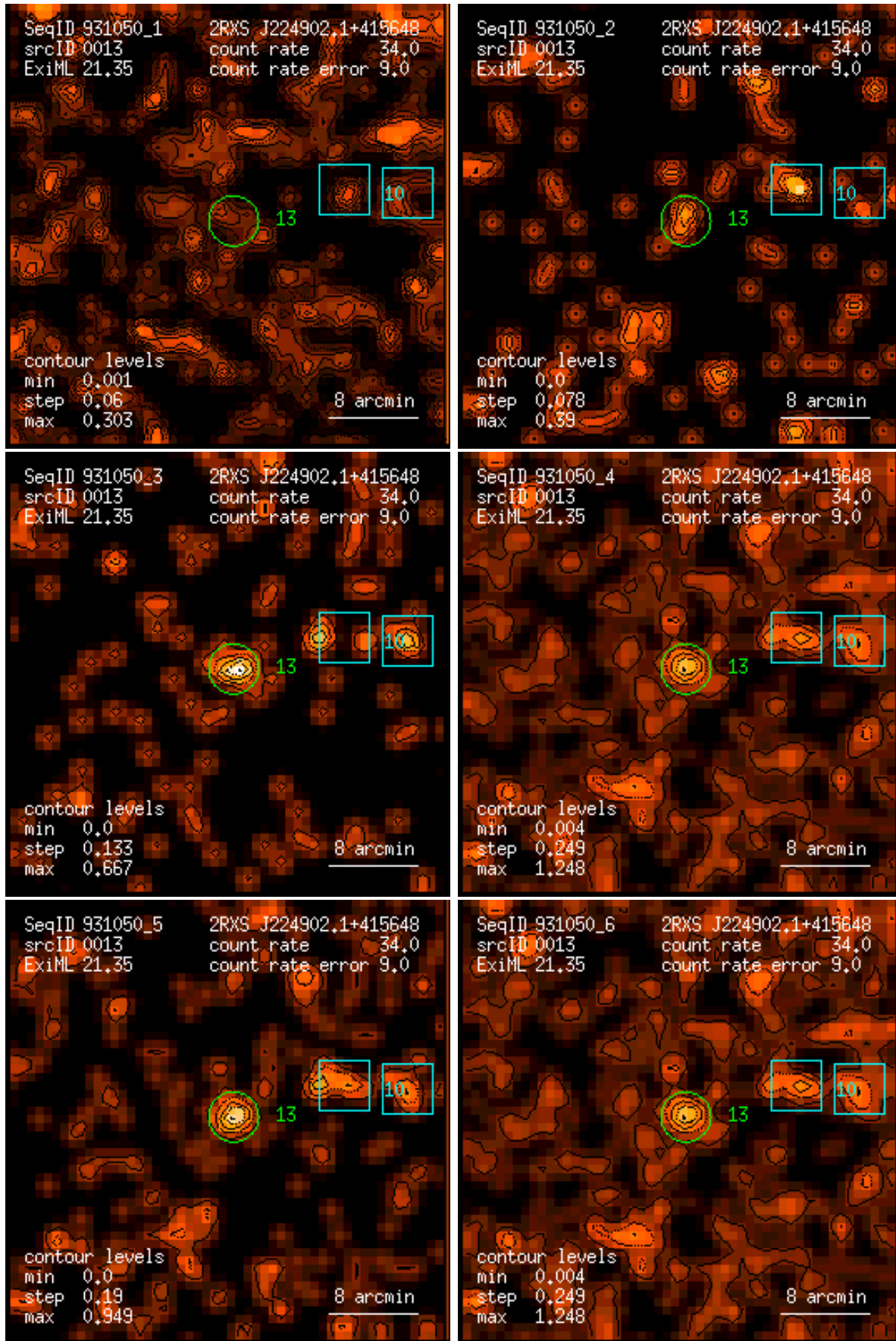
Figure 13: RASS 931050: detection 0013: band rate images, Gaussian filter: (1) PSPC channels 11 – 41, (2) 52 – 90, (3) 91 – 201, (4) 11 – 235, (5) 52 – 201, (6) 11 – 201. Broad band rates in counts/ks. Band rate contour levels in counts/ks/arcmin 2 .
