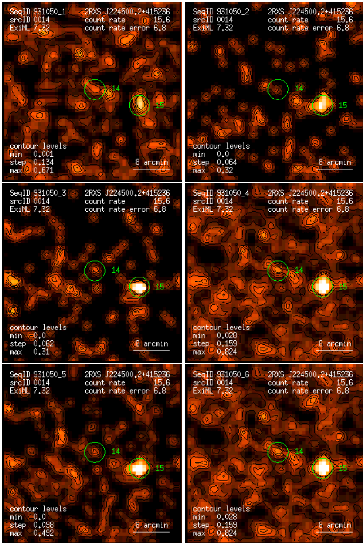
Figure 14: RASS 931050: detection 0014: band rate images, Gaussian filter: (1) PSPC channels 11 – 41, (2) 52 – 90, (3) 91 – 201, (4) 11 – 235, (5) 52 – 201, (6) 11 – 201. Broad band rates in counts/ks. Band rate contour levels in counts/ks/arcmin 2 .
