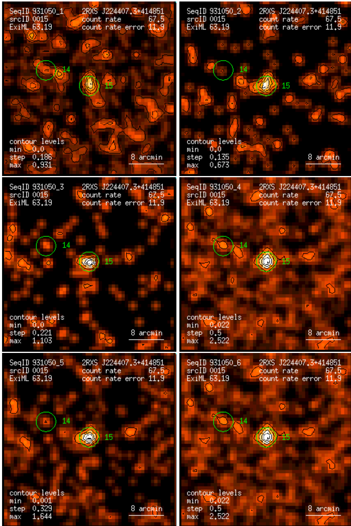
Figure 15: RASS 931050: detection 0015: band rate images, Gaussian filter: (1) PSPC channels 11 – 41, (2) 52 – 90, (3) 91 – 201, (4) 11 – 235, (5) 52 – 201, (6) 11 – 201. Broad band rates in counts/ks. Band rate contour levels in counts/ks/arcmin 2 .
