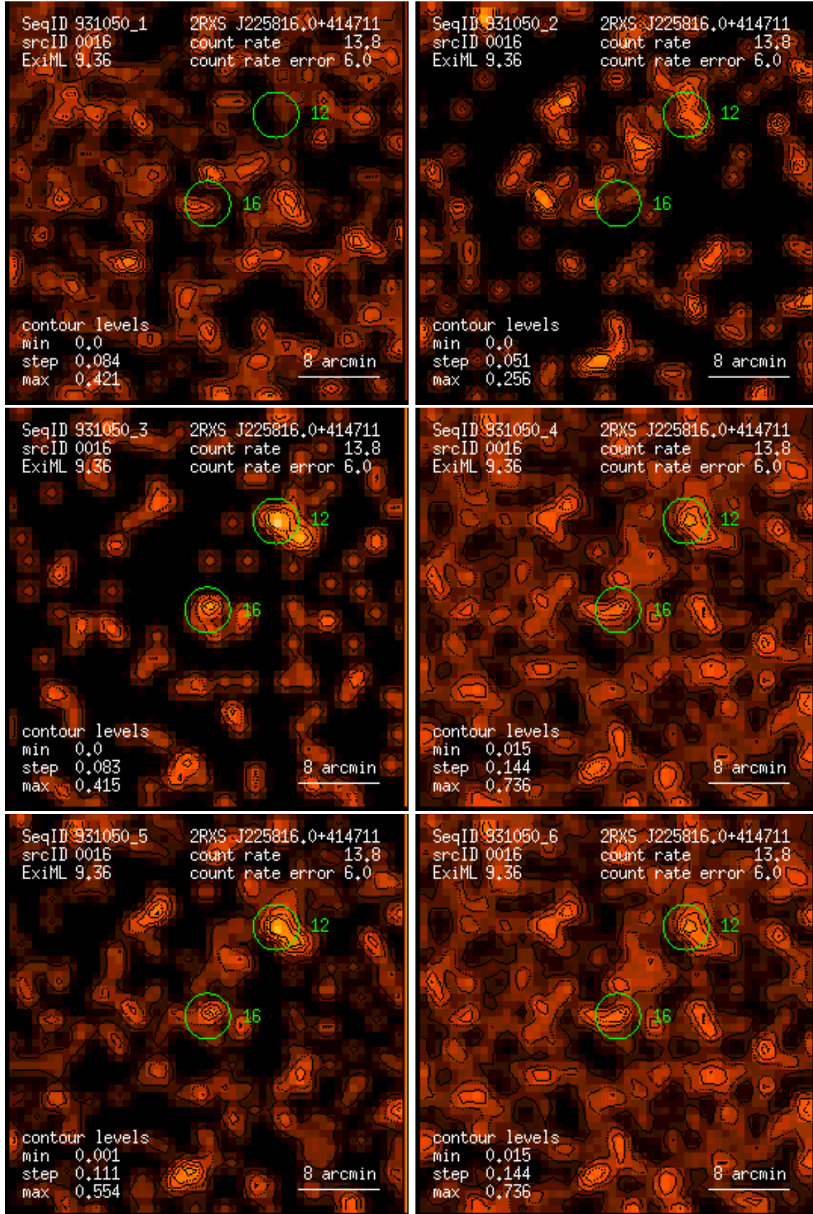
Figure 16: RASS 931050: detection 0016: band rate images, Gaussian filter: (1) PSPC channels 11 – 41, (2) 52 – 90, (3) 91 – 201, (4) 11 – 235, (5) 52 – 201, (6) 11 – 201. Broad band rates in counts/ks. Band rate contour levels in counts/ks/arcmin 2 .
