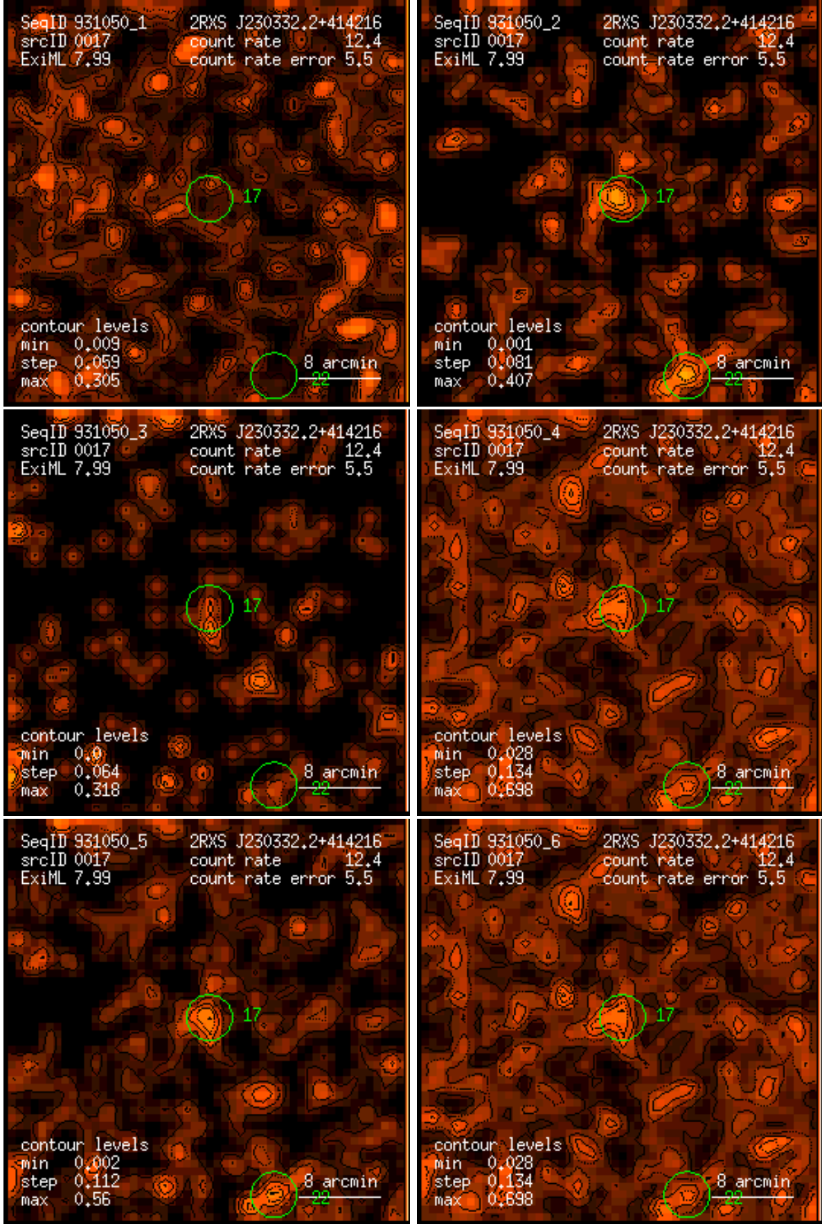
Figure 17: RASS 931050: detection 0017: band rate images, Gaussian filter: (1) PSPC channels 11 – 41, (2) 52 – 90, (3) 91 – 201, (4) 11 – 235, (5) 52 – 201, (6) 11 – 201. Broad band rates in counts/ks. Band rate contour levels in counts/ks/arcmin 2 .
