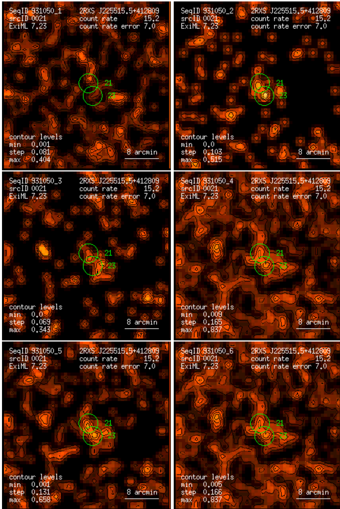
Figure 21: RASS 931050: detection 0021: band rate images, Gaussian filter: (1) PSPC channels 11 – 41, (2) 52 – 90, (3) 91 – 201, (4) 11 – 235, (5) 52 – 201, (6) 11 – 201. Broad band rates in counts/ks. Band rate contour levels in counts/ks/arcmin 2 .
