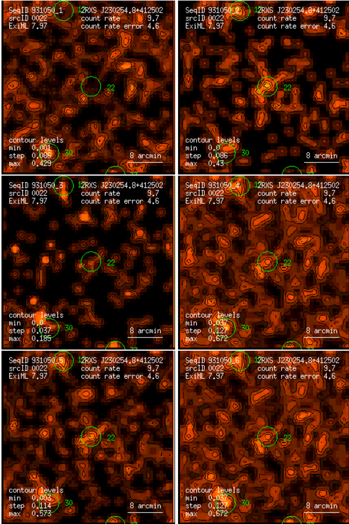
Figure 22: RASS 931050: detection 0022: band rate images, Gaussian filter: (1) PSPC channels 11 – 41, (2) 52 – 90, (3) 91 – 201, (4) 11 – 235, (5) 52 – 201, (6) 11 – 201. Broad band rates in counts/ks. Band rate contour levels in counts/ks/arcmin 2 .
