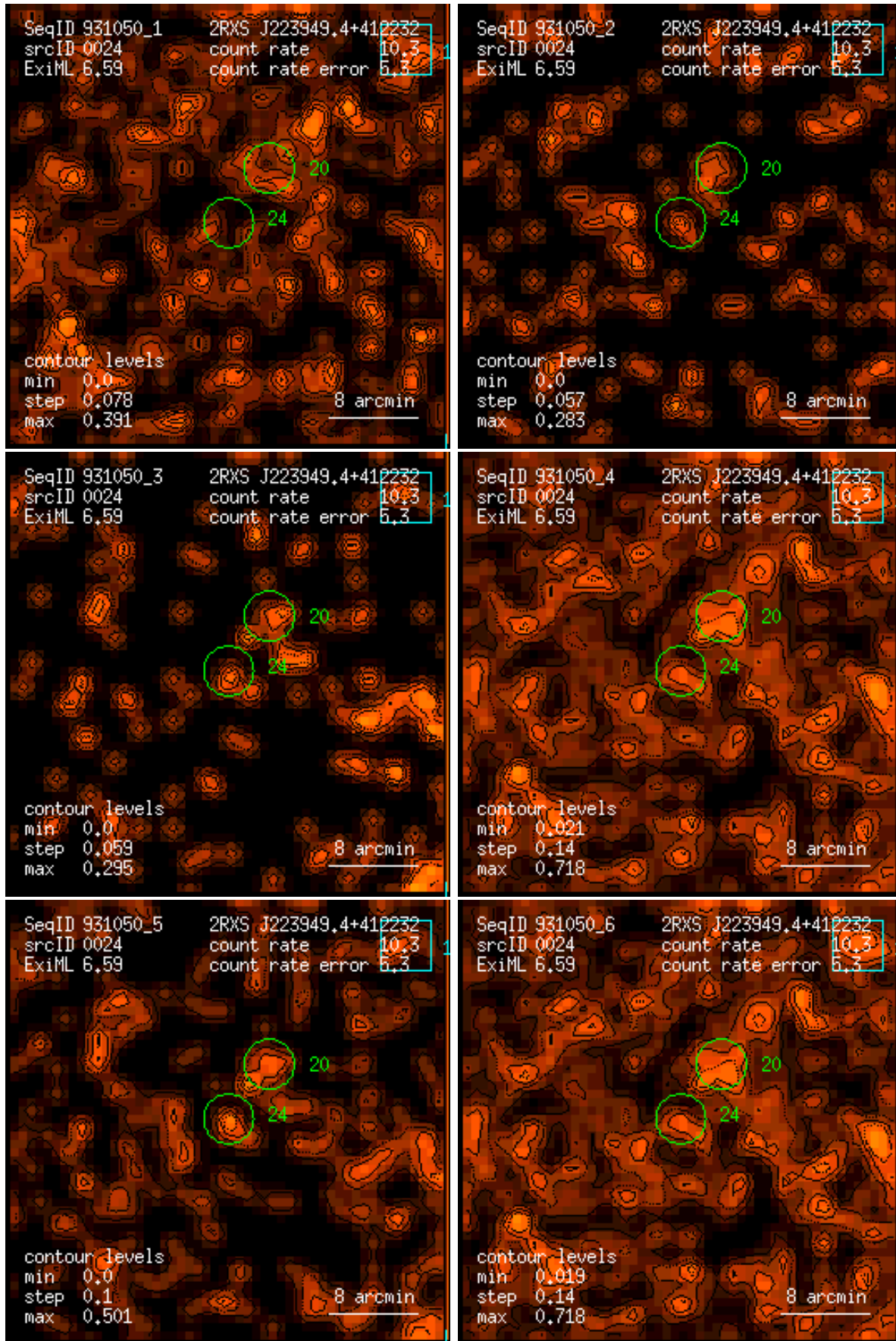
Figure 24: RASS 931050: detection 0024: band rate images, Gaussian filter: (1) PSPC channels 11 – 41, (2) 52 – 90, (3) 91 – 201, (4) 11 – 235, (5) 52 – 201, (6) 11 – 201. Broad band rates in counts/ks. Band rate contour levels in counts/ks/arcmin 2 .
