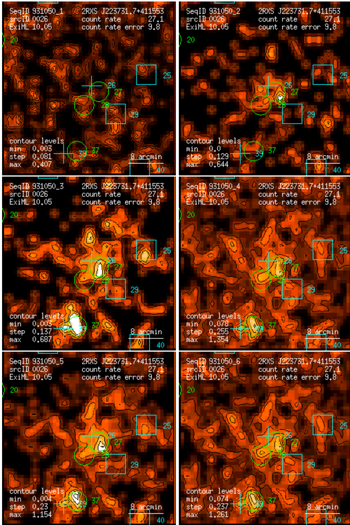
Figure 26: RASS 931050: detection 0026: band rate images, Gaussian filter: (1) PSPC channels 11 – 41, (2) 52 – 90, (3) 91 – 201, (4) 11 – 235, (5) 52 – 201, (6) 11 – 201. Broad band rates in counts/ks. Band rate contour levels in counts/ks/arcmin 2 .
