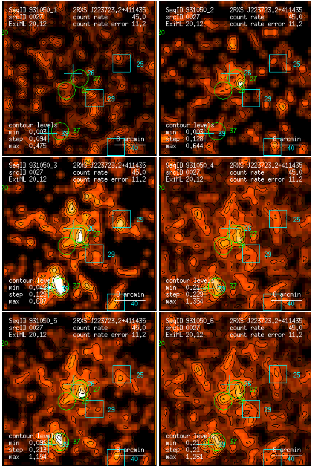
Figure 27: RASS 931050: detection 0027: band rate images, Gaussian filter: (1) PSPC channels 11 – 41, (2) 52 – 90, (3) 91 – 201, (4) 11 – 235, (5) 52 – 201, (6) 11 – 201. Broad band rates in counts/ks. Band rate contour levels in counts/ks/arcmin 2 .
