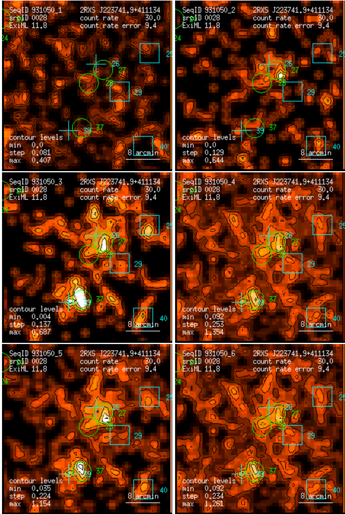
Figure 28: RASS 931050: detection 0028: band rate images, Gaussian filter: (1) PSPC channels 11 – 41, (2) 52 – 90, (3) 91 – 201, (4) 11 – 235, (5) 52 – 201, (6) 11 – 201. Broad band rates in counts/ks. Band rate contour levels in counts/ks/arcmin 2 .
