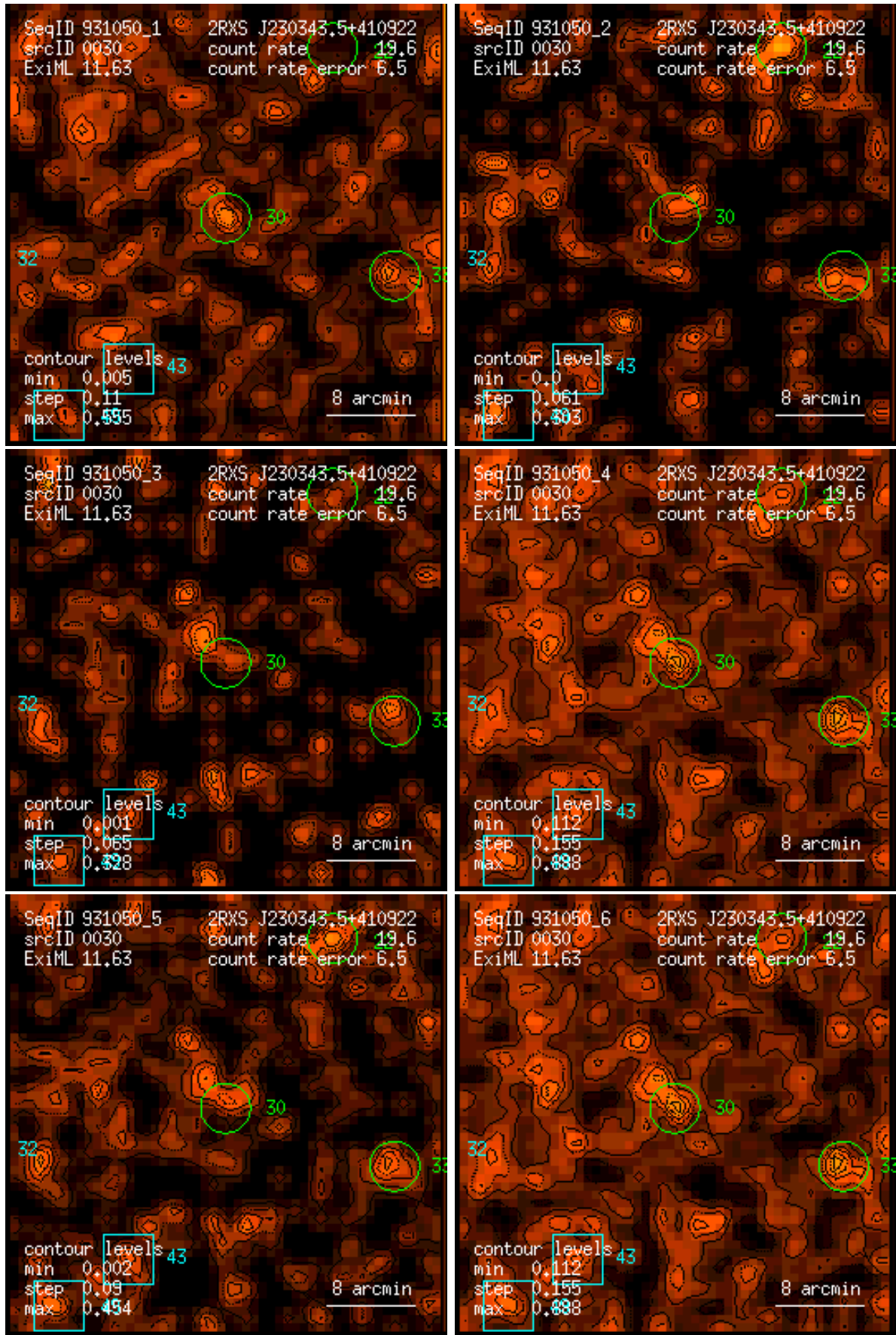
Figure 30: RASS 931050: detection 0030: band rate images, Gaussian filter: (1) PSPC channels 11 – 41, (2) 52 – 90, (3) 91 – 201, (4) 11 – 235, (5) 52 – 201, (6) 11 – 201. Broad band rates in counts/ks. Band rate contour levels in counts/ks/arcmin 2 .
