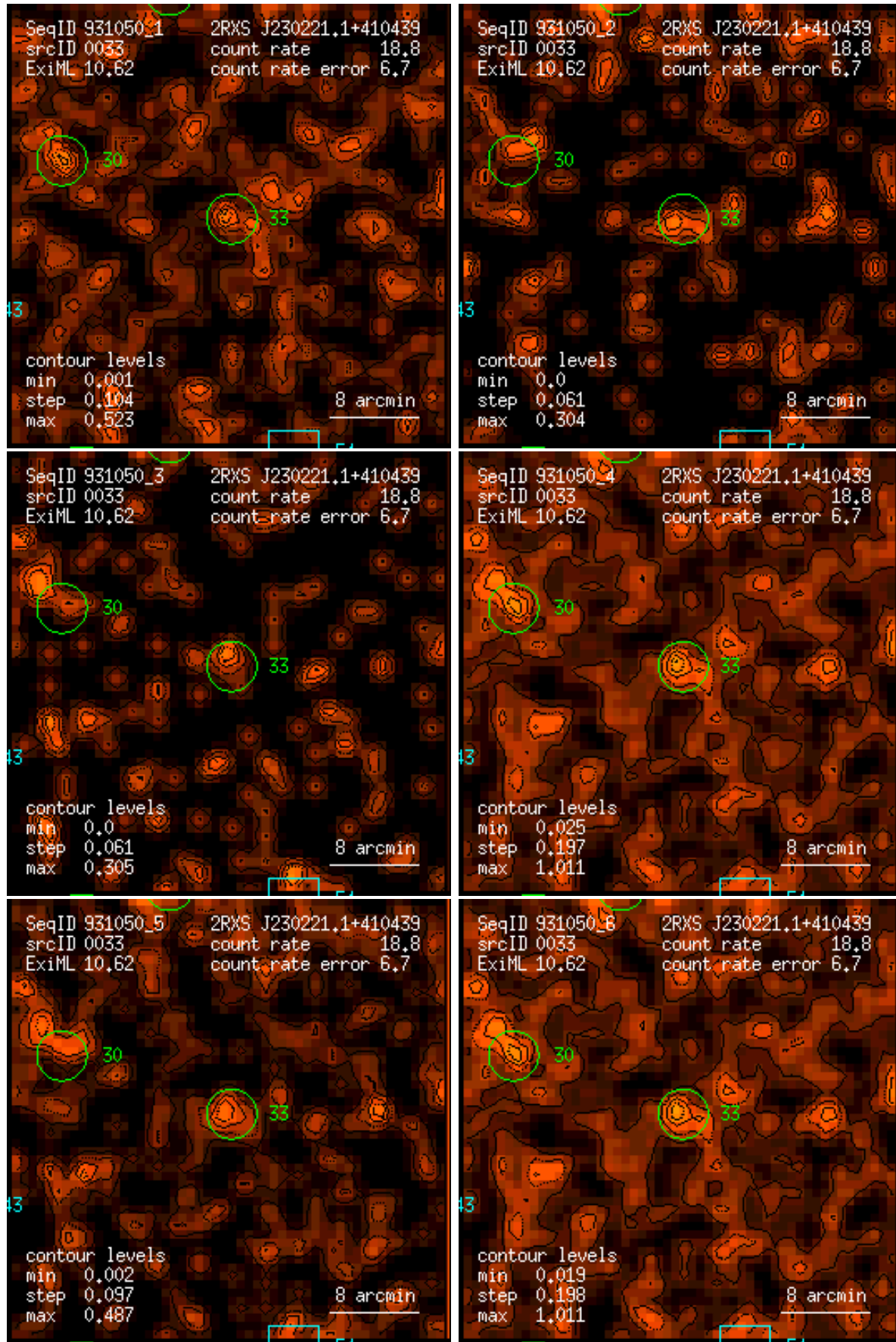
Figure 33: RASS 931050: detection 0033: band rate images, Gaussian filter: (1) PSPC channels 11 – 41, (2) 52 – 90, (3) 91 – 201, (4) 11 – 235, (5) 52 – 201, (6) 11 – 201. Broad band rates in counts/ks. Band rate contour levels in counts/ks/arcmin 2 .
