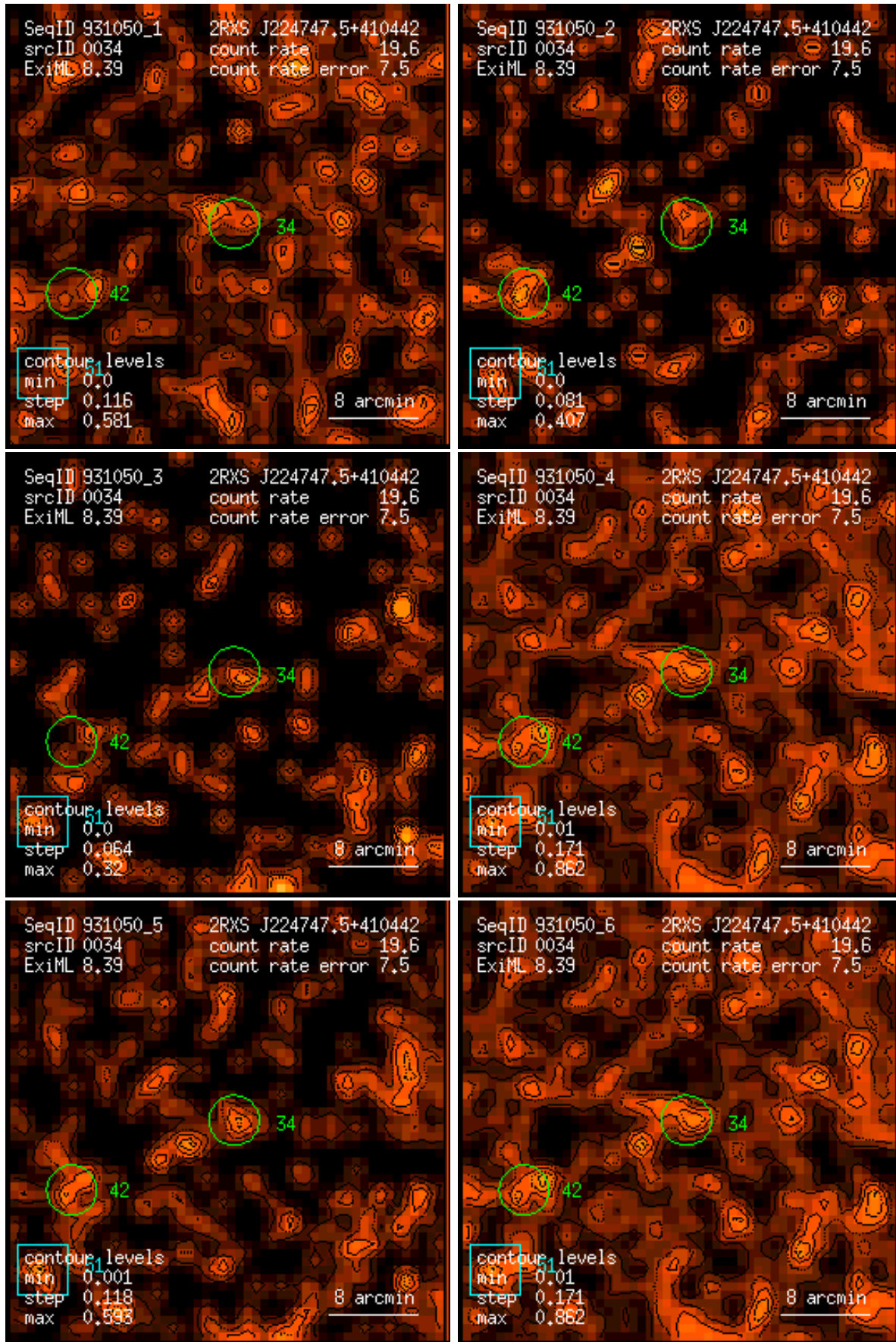
Figure 34: RASS 931050: detection 0034: band rate images, Gaussian filter: (1) PSPC channels 11 – 41, (2) 52 – 90, (3) 91 – 201, (4) 11 – 235, (5) 52 – 201, (6) 11 – 201. Broad band rates in counts/ks. Band rate contour levels in counts/ks/arcmin 2 .
