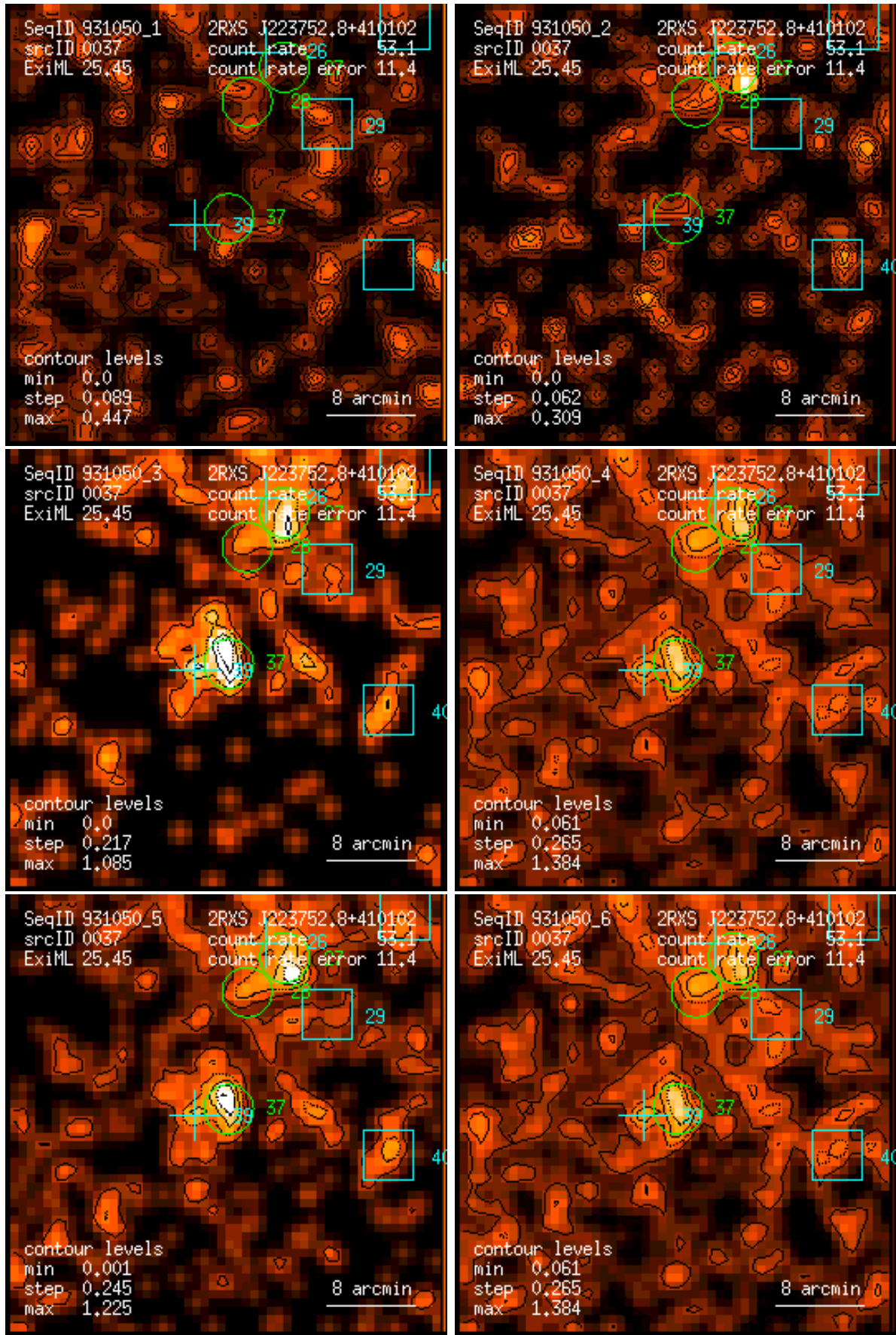
Figure 37: RASS 931050: detection 0037: band rate images, Gaussian filter: (1) PSPC channels 11 – 41, (2) 52 – 90, (3) 91 – 201, (4) 11 – 235, (5) 52 – 201, (6) 11 – 201. Broad band rates in counts/ks. Band rate contour levels in counts/ks/arcmin 2 .
