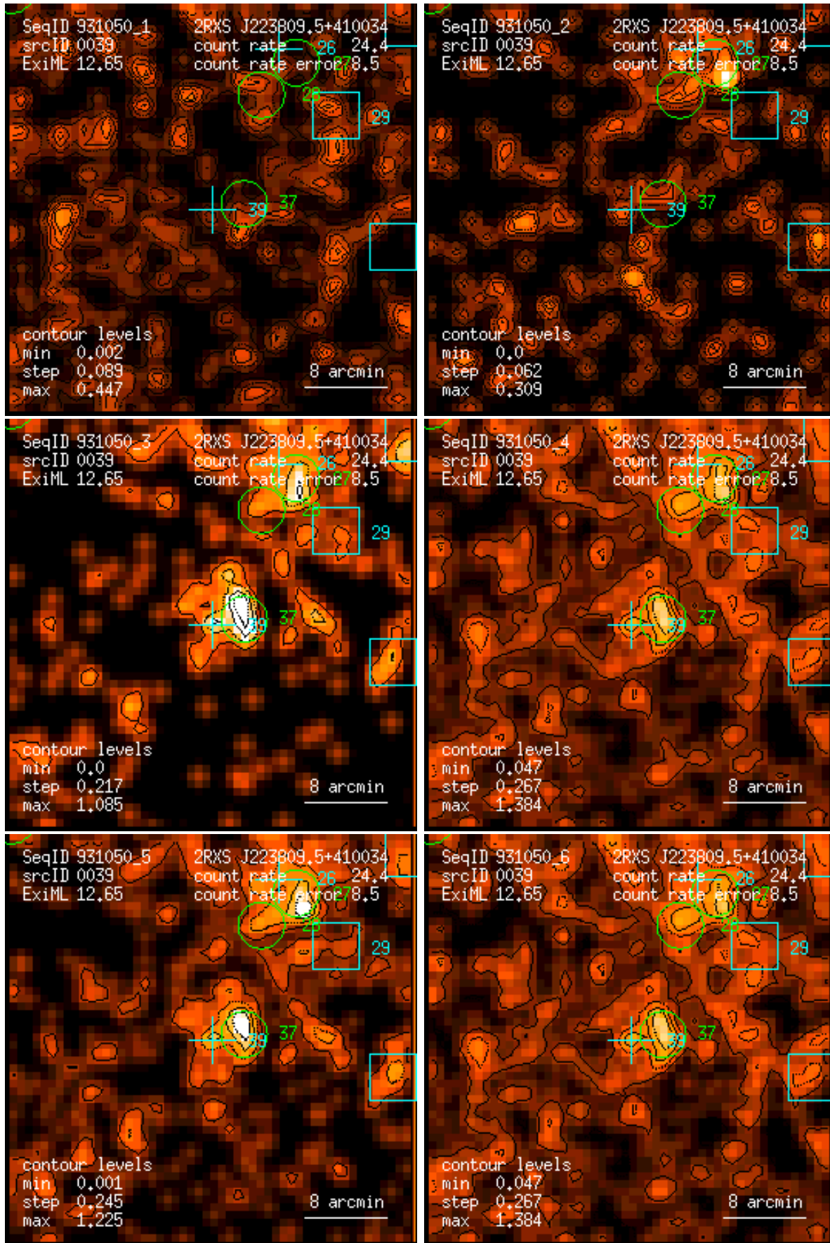
Figure 39: RASS 931050: detection 0039: band rate images, Gaussian filter: (1) PSPC channels 11 – 41, (2) 52 – 90, (3) 91 – 201, (4) 11 – 235, (5) 52 – 201, (6) 11 – 201. Broad band rates in counts/ks. Band rate contour levels in counts/ks/arcmin 2 .
