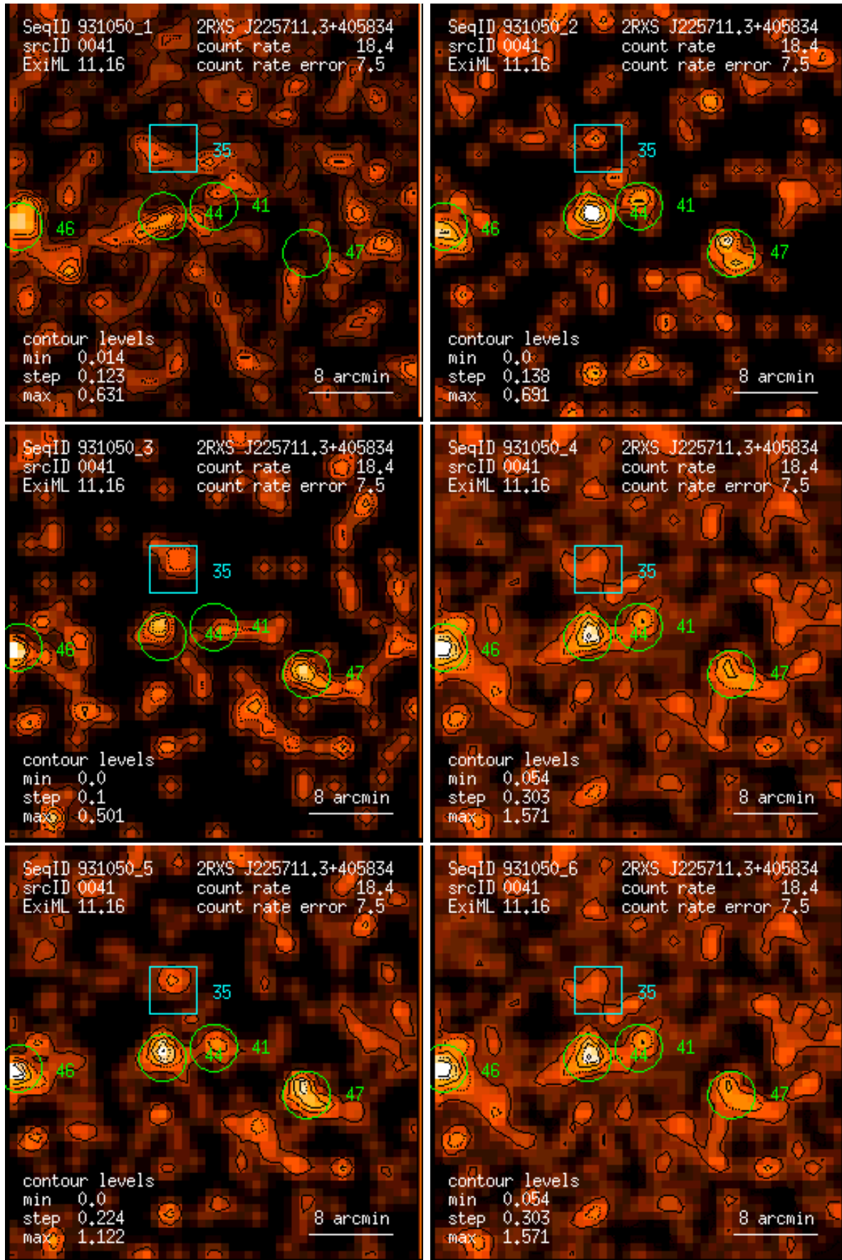
Figure 41: RASS 931050: detection 0041: band rate images, Gaussian filter: (1) PSPC channels 11 – 41, (2) 52 – 90, (3) 91 – 201, (4) 11 – 235, (5) 52 – 201, (6) 11 – 201. Broad band rates in counts/ks. Band rate contour levels in counts/ks/arcmin 2 .
