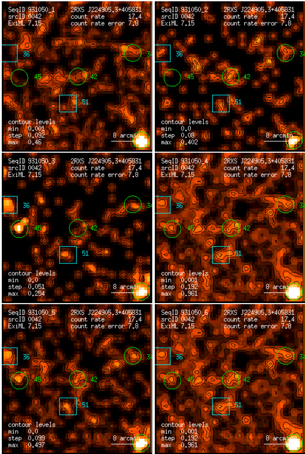
Figure 42: RASS 931050: detection 0042: band rate images, Gaussian filter: (1) PSPC channels 11 – 41, (2) 52 – 90, (3) 91 – 201, (4) 11 – 235, (5) 52 – 201, (6) 11 – 201. Broad band rates in counts/ks. Band rate contour levels in counts/ks/arcmin 2 .
