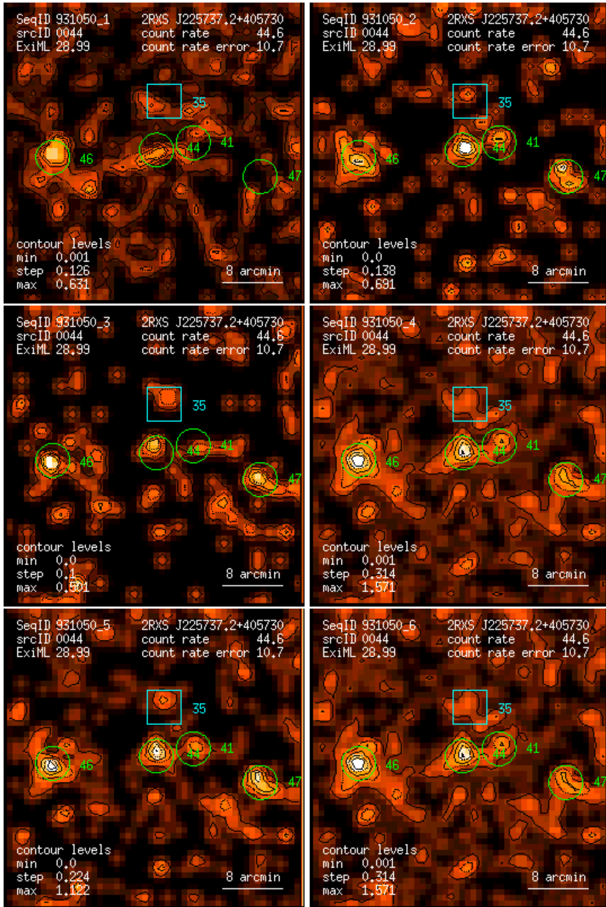
Figure 44: RASS 931050: detection 0044: band rate images, Gaussian filter: (1) PSPC channels 11 – 41, (2) 52 – 90, (3) 91 – 201, (4) 11 – 235, (5) 52 – 201, (6) 11 – 201. Broad band rates in counts/ks. Band rate contour levels in counts/ks/arcmin 2 .
