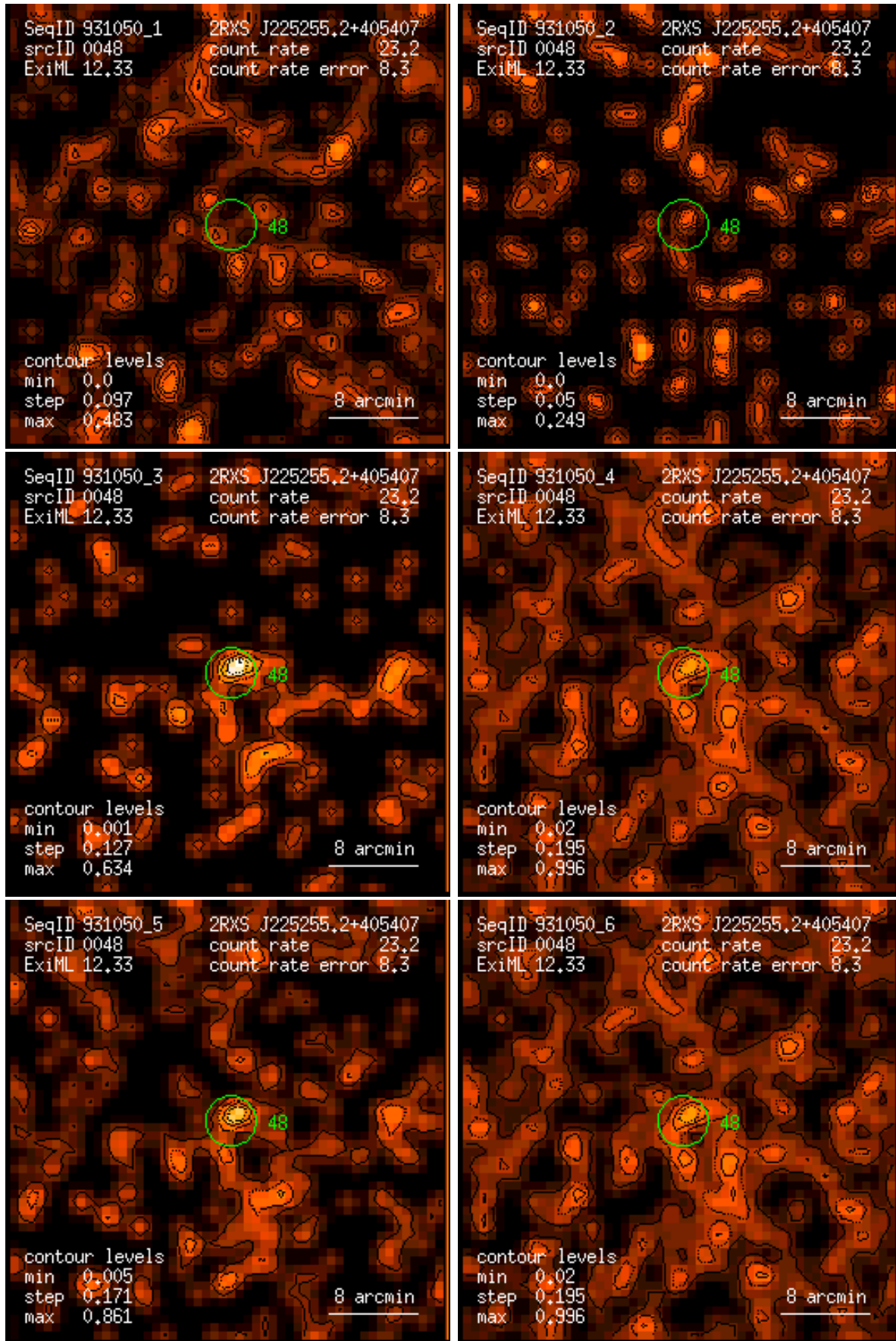
Figure 48: RASS 931050: detection 0048: band rate images, Gaussian filter: (1) PSPC channels 11 – 41, (2) 52 – 90, (3) 91 – 201, (4) 11 – 235, (5) 52 – 201, (6) 11 – 201. Broad band rates in counts/ks. Band rate contour levels in counts/ks/arcmin 2 .
