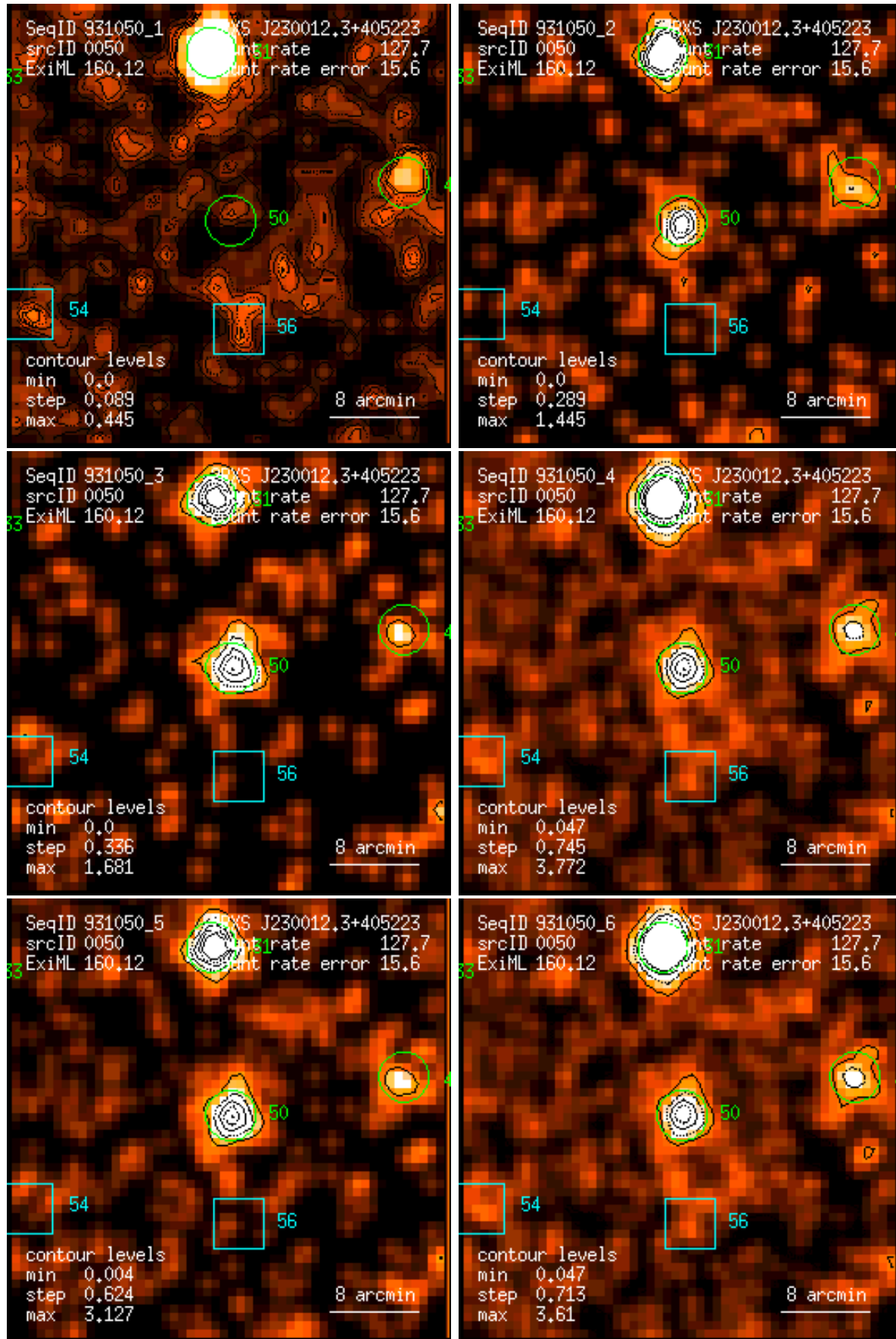
Figure 50: RASS 931050: detection 0050: band rate images, Gaussian filter: (1) PSPC channels 11 – 41, (2) 52 – 90, (3) 91 – 201, (4) 11 – 235, (5) 52 – 201, (6) 11 – 201. Broad band rates in counts/ks. Band rate contour levels in counts/ks/arcmin 2 .
