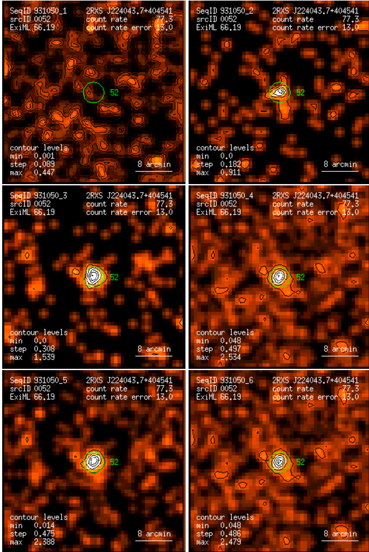
Figure 52: RASS 931050: detection 0052: band rate images, Gaussian filter: (1) PSPC channels 11 – 41, (2) 52 – 90, (3) 91 – 201, (4) 11 – 235, (5) 52 – 201, (6) 11 – 201. Broad band rates in counts/ks. Band rate contour levels in counts/ks/arcmin 2 .
