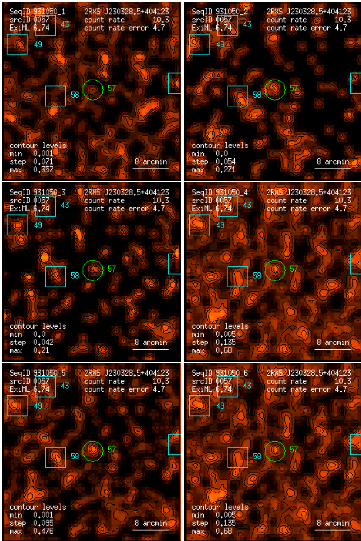
Figure 57: RASS 931050: detection 0057: band rate images, Gaussian filter: (1) PSPC channels 11 – 41, (2) 52 – 90, (3) 91 – 201, (4) 11 – 235, (5) 52 – 201, (6) 11 – 201. Broad band rates in counts/ks. Band rate contour levels in counts/ks/arcmin 2 .
