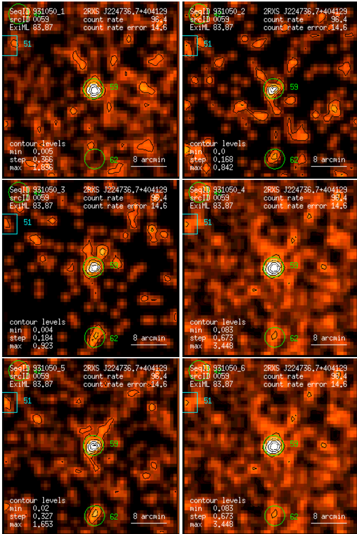
Figure 59: RASS 931050: detection 0059: band rate images, Gaussian filter: (1) PSPC channels 11 – 41, (2) 52 – 90, (3) 91 – 201, (4) 11 – 235, (5) 52 – 201, (6) 11 – 201. Broad band rates in counts/ks. Band rate contour levels in counts/ks/arcmin 2 .
