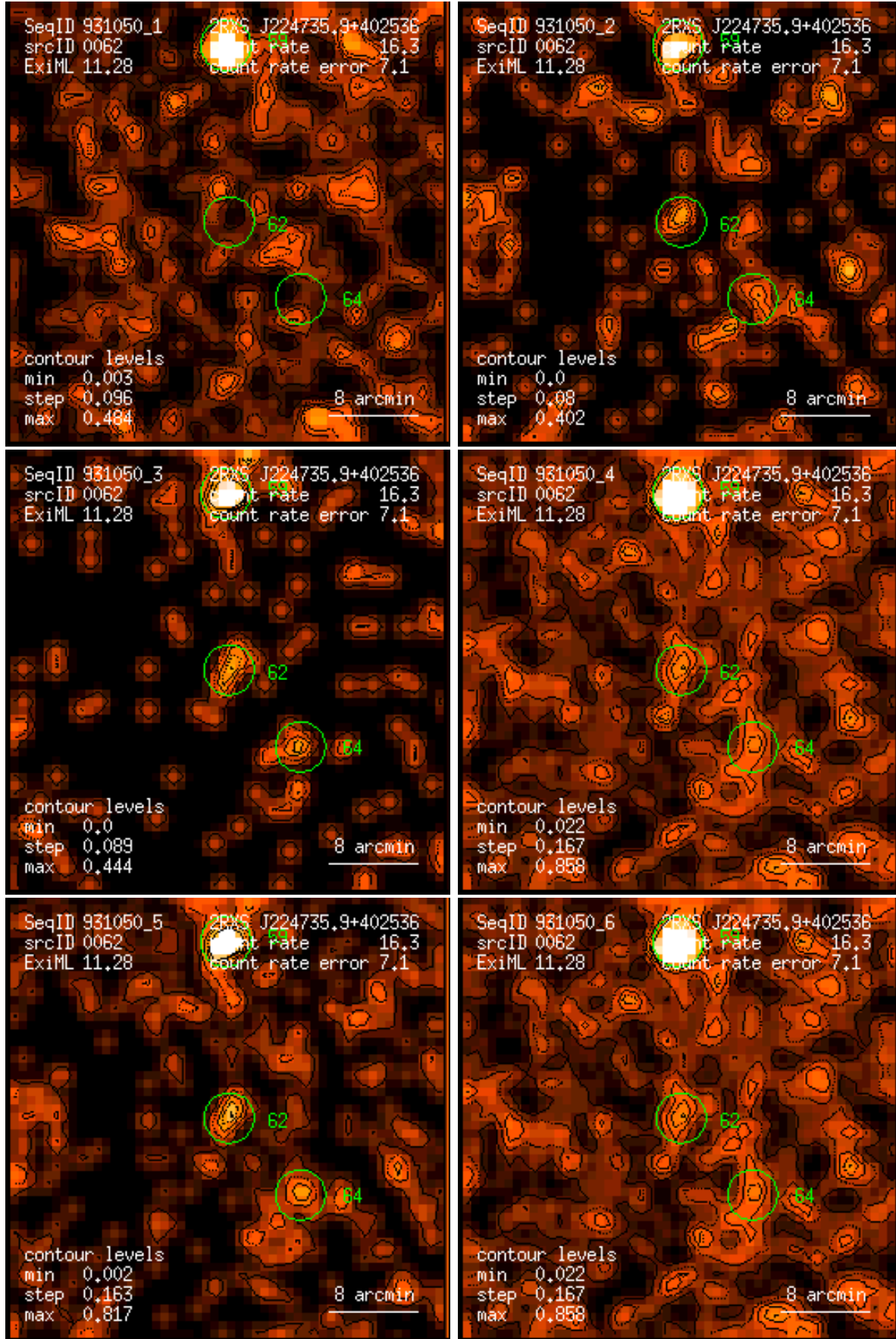
Figure 62: RASS 931050: detection 0062: band rate images, Gaussian filter: (1) PSPC channels 11 – 41, (2) 52 – 90, (3) 91 – 201, (4) 11 – 235, (5) 52 – 201, (6) 11 – 201. Broad band rates in counts/ks. Band rate contour levels in counts/ks/arcmin 2 .
