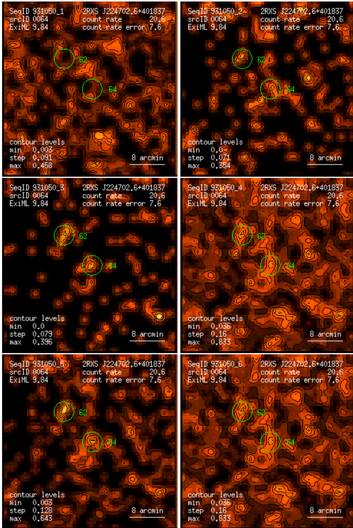
Figure 64: RASS 931050: detection 0064: band rate images, Gaussian filter: (1) PSPC channels 11 – 41, (2) 52 – 90, (3) 91 – 201, (4) 11 – 235, (5) 52 – 201, (6) 11 – 201. Broad band rates in counts/ks. Band rate contour levels in counts/ks/arcmin 2 .
