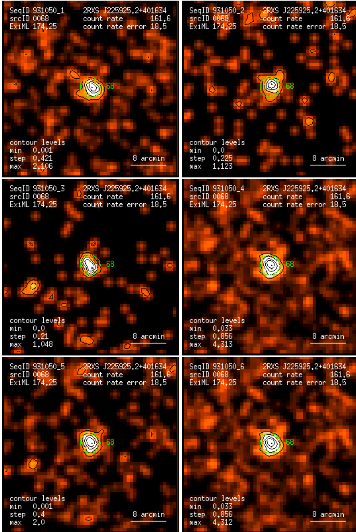
Figure 68: RASS 931050: detection 0068: band rate images, Gaussian filter: (1) PSPC channels 11 – 41, (2) 52 – 90, (3) 91 – 201, (4) 11 – 235, (5) 52 – 201, (6) 11 – 201. Broad band rates in counts/ks. Band rate contour levels in counts/ks/arcmin 2 .
