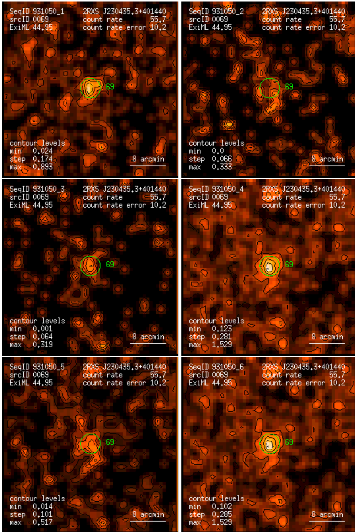
Figure 69: RASS 931050: detection 0069: band rate images, Gaussian filter: (1) PSPC channels 11 – 41, (2) 52 – 90, (3) 91 – 201, (4) 11 – 235, (5) 52 – 201, (6) 11 – 201. Broad band rates in counts/ks. Band rate contour levels in counts/ks/arcmin 2 .
