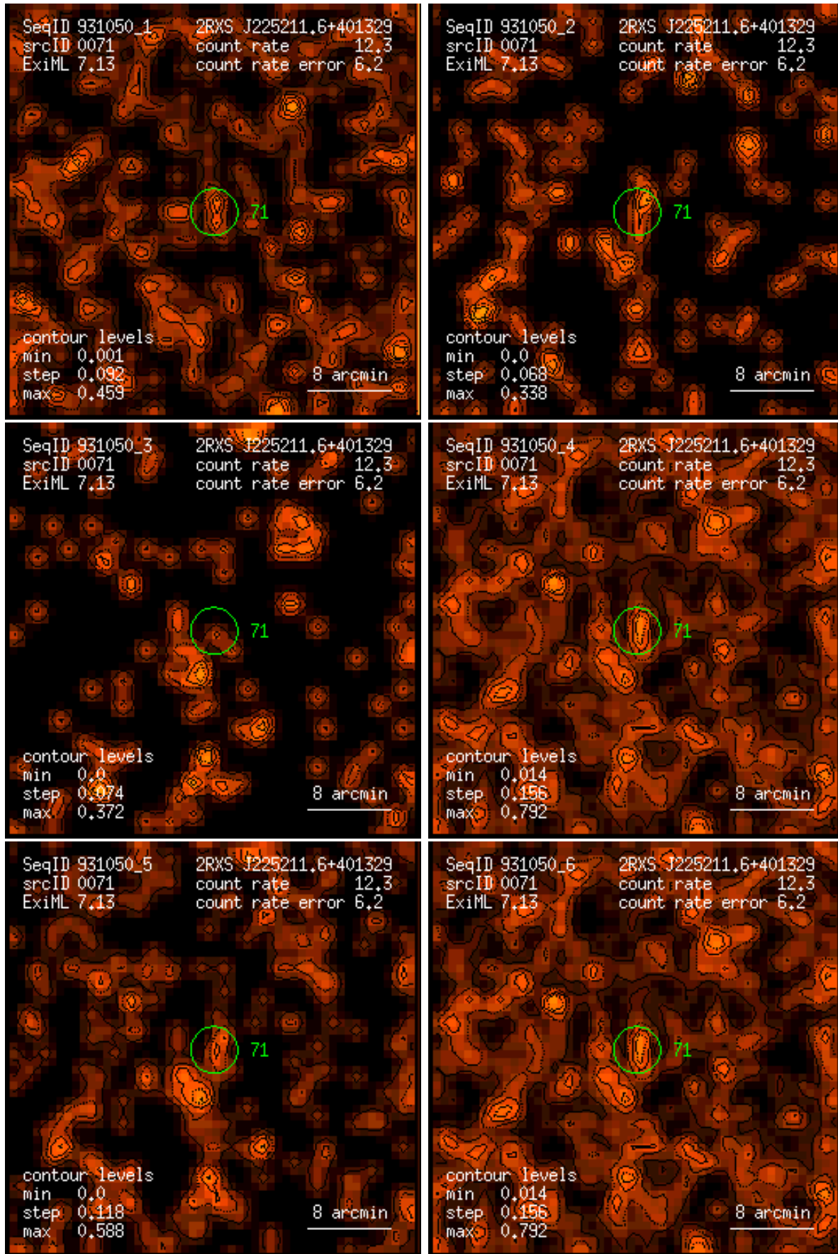
Figure 71: RASS 931050: detection 0071: band rate images, Gaussian filter: (1) PSPC channels 11 – 41, (2) 52 – 90, (3) 91 – 201, (4) 11 – 235, (5) 52 – 201, (6) 11 – 201. Broad band rates in counts/ks. Band rate contour levels in counts/ks/arcmin 2 .
