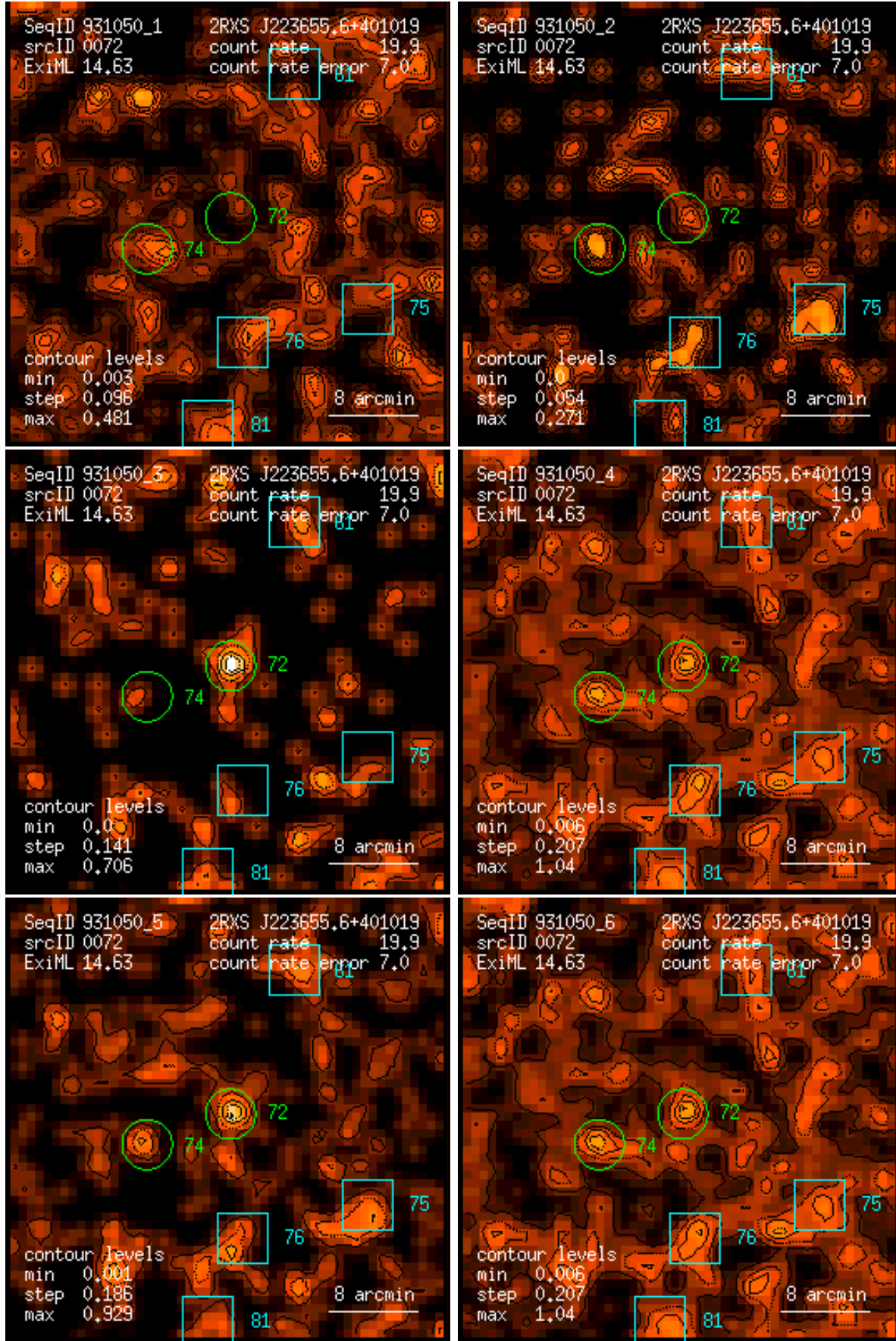
Figure 72: RASS 931050: detection 0072: band rate images, Gaussian filter: (1) PSPC channels 11 – 41, (2) 52 – 90, (3) 91 – 201, (4) 11 – 235, (5) 52 – 201, (6) 11 – 201. Broad band rates in counts/ks. Band rate contour levels in counts/ks/arcmin 2 .
